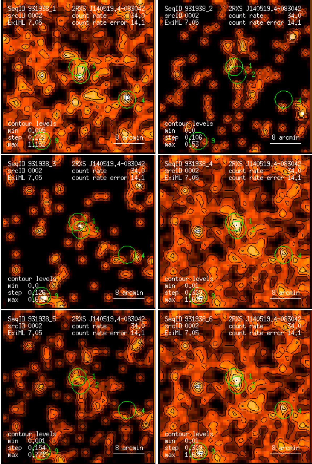
Figure 2: RASS 931938: detection 0002: band rate images, Gaussian filter: (1) PSPC channels 11 – 41, (2) 52 – 90, (3) 91 – 201, (4) 11 – 235, (5) 52 – 201, (6) 11 – 201. Broad band rates in counts/ks. Band rate contour levels in counts/ks/arcmin 2 .
