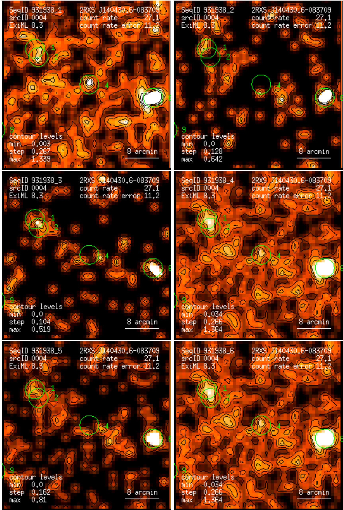
Figure 4: RASS 931938: detection 0004: band rate images, Gaussian filter: (1) PSPC channels 11 – 41, (2) 52 – 90, (3) 91 – 201, (4) 11 – 235, (5) 52 – 201, (6) 11 – 201. Broad band rates in counts/ks. Band rate contour levels in counts/ks/arcmin 2 .
