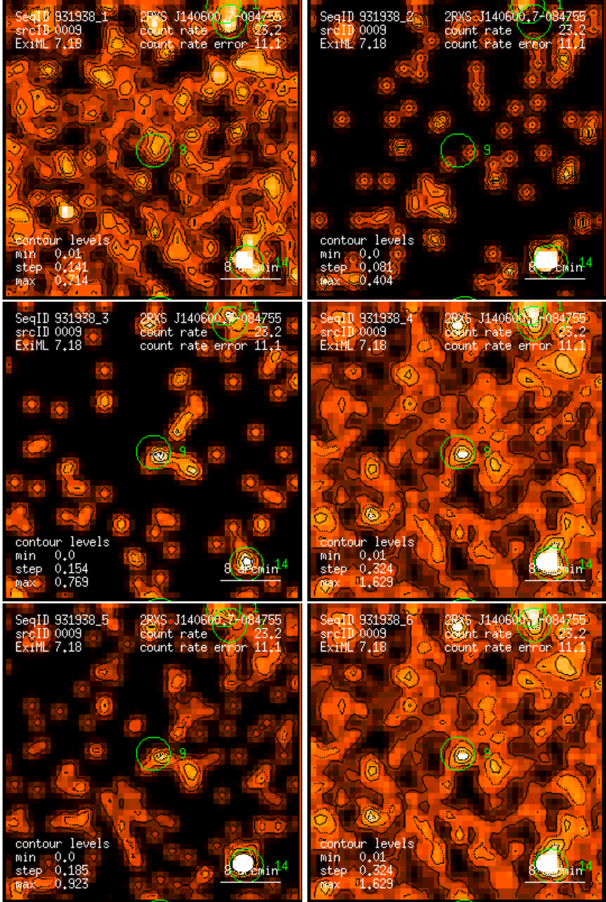
Figure 9: RASS 931938: detection 0009: band rate images, Gaussian filter: (1) PSPC channels 11 – 41, (2) 52 – 90, (3) 91 – 201, (4) 11 – 235, (5) 52 – 201, (6) 11 – 201. Broad band rates in counts/ks. Band rate contour levels in counts/ks/arcmin 2 .
