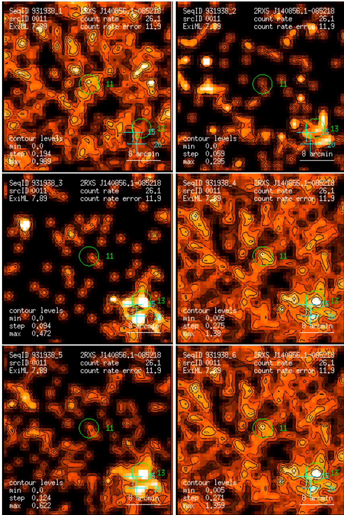
Figure 11: RASS 931938: detection 0011: band rate images, Gaussian filter: (1) PSPC channels 11 – 41, (2) 52 – 90, (3) 91 – 201, (4) 11 – 235, (5) 52 – 201, (6) 11 – 201. Broad band rates in counts/ks. Band rate contour levels in counts/ks/arcmin 2 .
