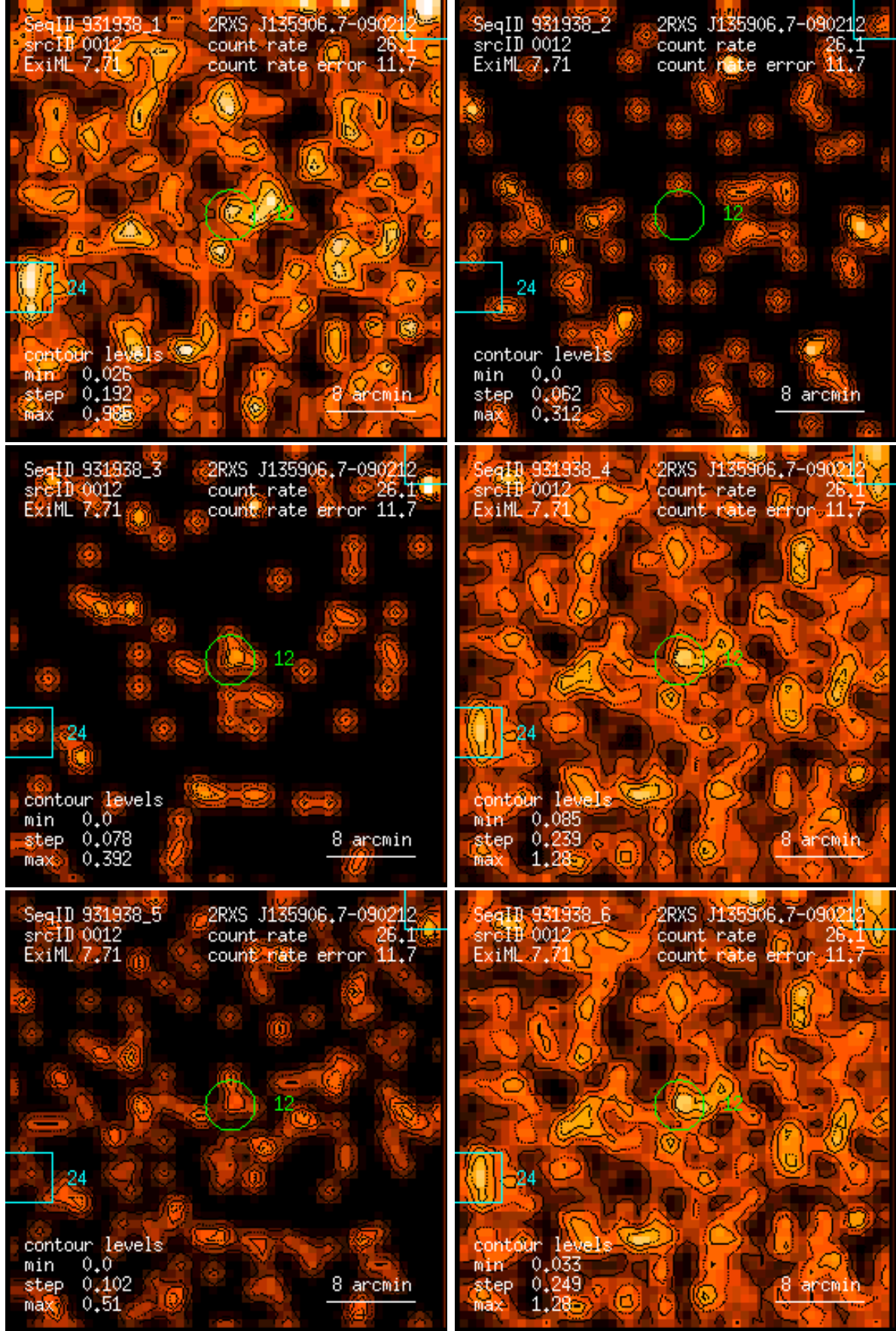
Figure 12: RASS 931938: detection 0012: band rate images, Gaussian filter: (1) PSPC channels 11 – 41, (2) 52 – 90, (3) 91 – 201, (4) 11 – 235, (5) 52 – 201, (6) 11 – 201. Broad band rates in counts/ks. Band rate contour levels in counts/ks/arcmin 2 .
