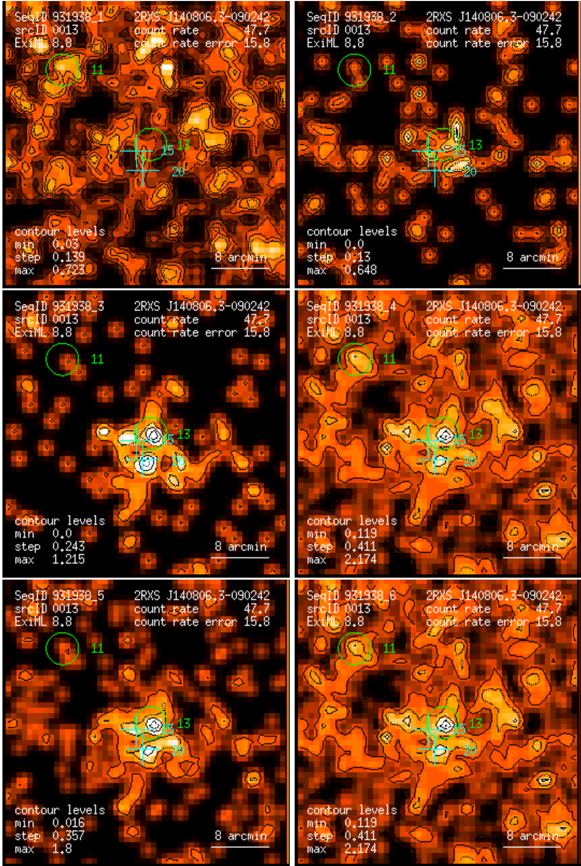
Figure 13: RASS 931938: detection 0013: band rate images, Gaussian filter: (1) PSPC channels 11 – 41, (2) 52 – 90, (3) 91 – 201, (4) 11 – 235, (5) 52 – 201, (6) 11 – 201. Broad band rates in counts/ks. Band rate contour levels in counts/ks/arcmin 2 .
