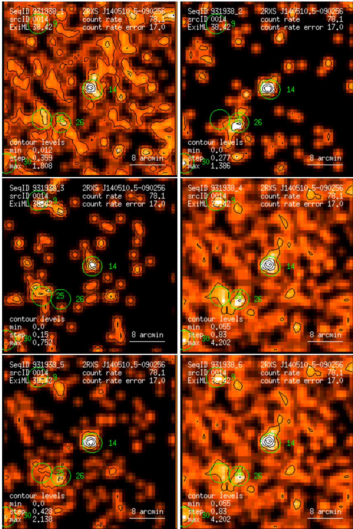
Figure 14: RASS 931938: detection 0014: band rate images, Gaussian filter: (1) PSPC channels 11 – 41, (2) 52 – 90, (3) 91 – 201, (4) 11 – 235, (5) 52 – 201, (6) 11 – 201. Broad band rates in counts/ks. Band rate contour levels in counts/ks/arcmin 2 .
