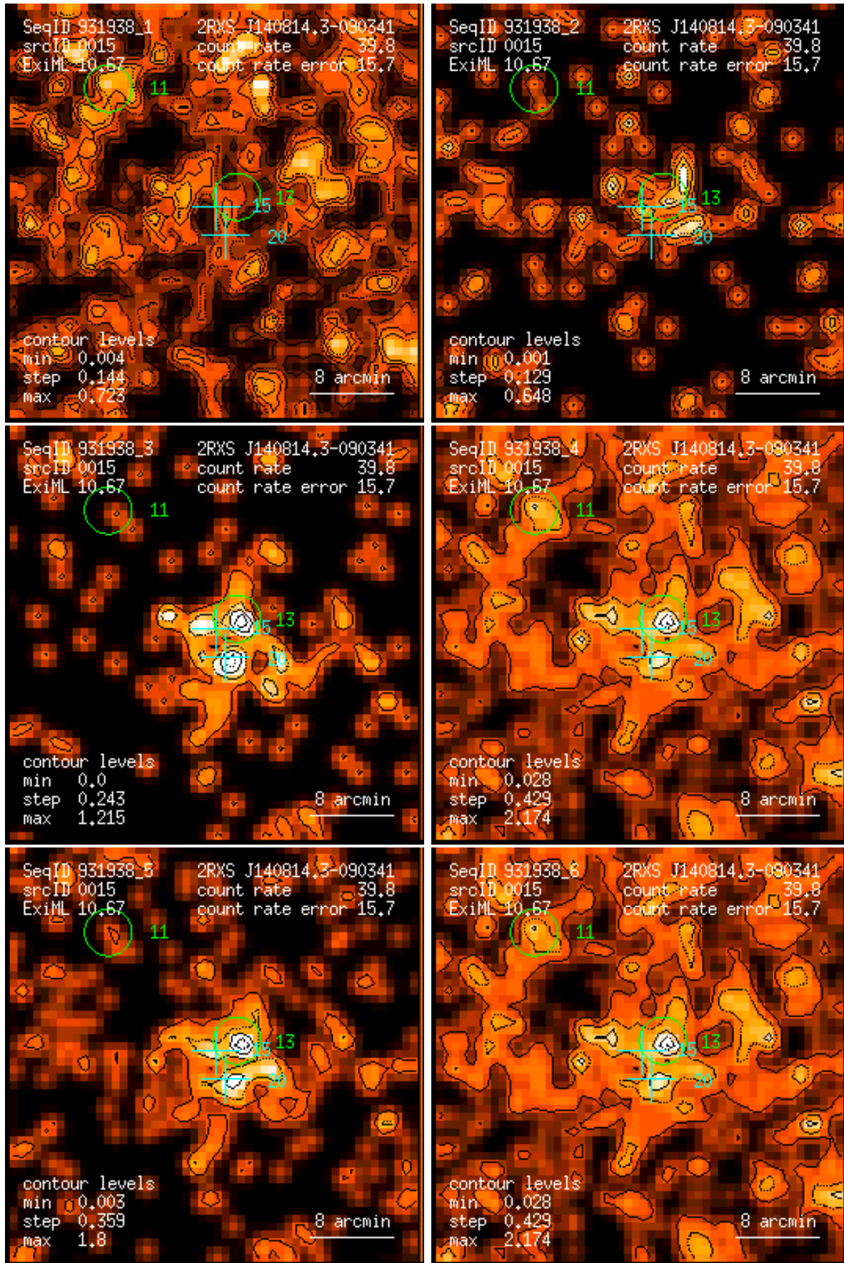
Figure 15: RASS 931938: detection 0015: band rate images, Gaussian filter: (1) PSPC channels 11 – 41, (2) 52 – 90, (3) 91 – 201, (4) 11 – 235, (5) 52 – 201, (6) 11 – 201. Broad band rates in counts/ks. Band rate contour levels in counts/ks/arcmin 2 .
