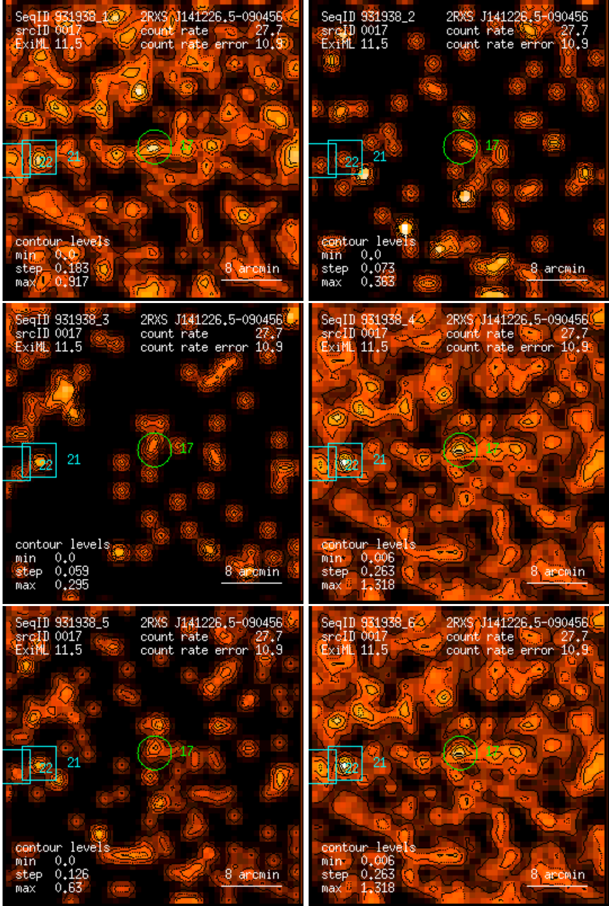
Figure 17: RASS 931938: detection 0017: band rate images, Gaussian filter: (1) PSPC channels 11 – 41, (2) 52 – 90, (3) 91 – 201, (4) 11 – 235, (5) 52 – 201, (6) 11 – 201. Broad band rates in counts/ks. Band rate contour levels in counts/ks/arcmin 2 .
