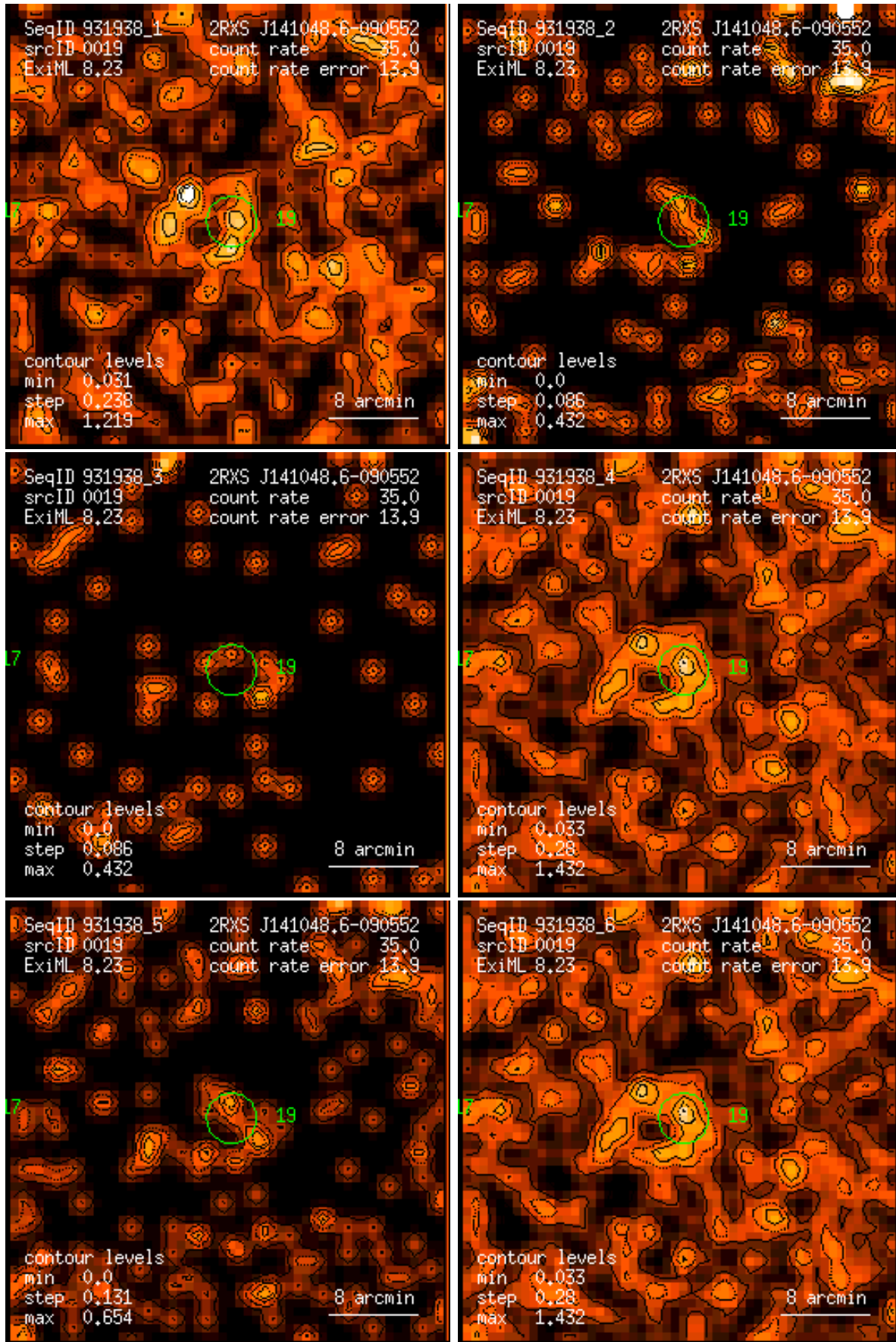
Figure 19: RASS 931938: detection 0019: band rate images, Gaussian filter: (1) PSPC channels 11 – 41, (2) 52 – 90, (3) 91 – 201, (4) 11 – 235, (5) 52 – 201, (6) 11 – 201. Broad band rates in counts/ks. Band rate contour levels in counts/ks/arcmin 2 .
