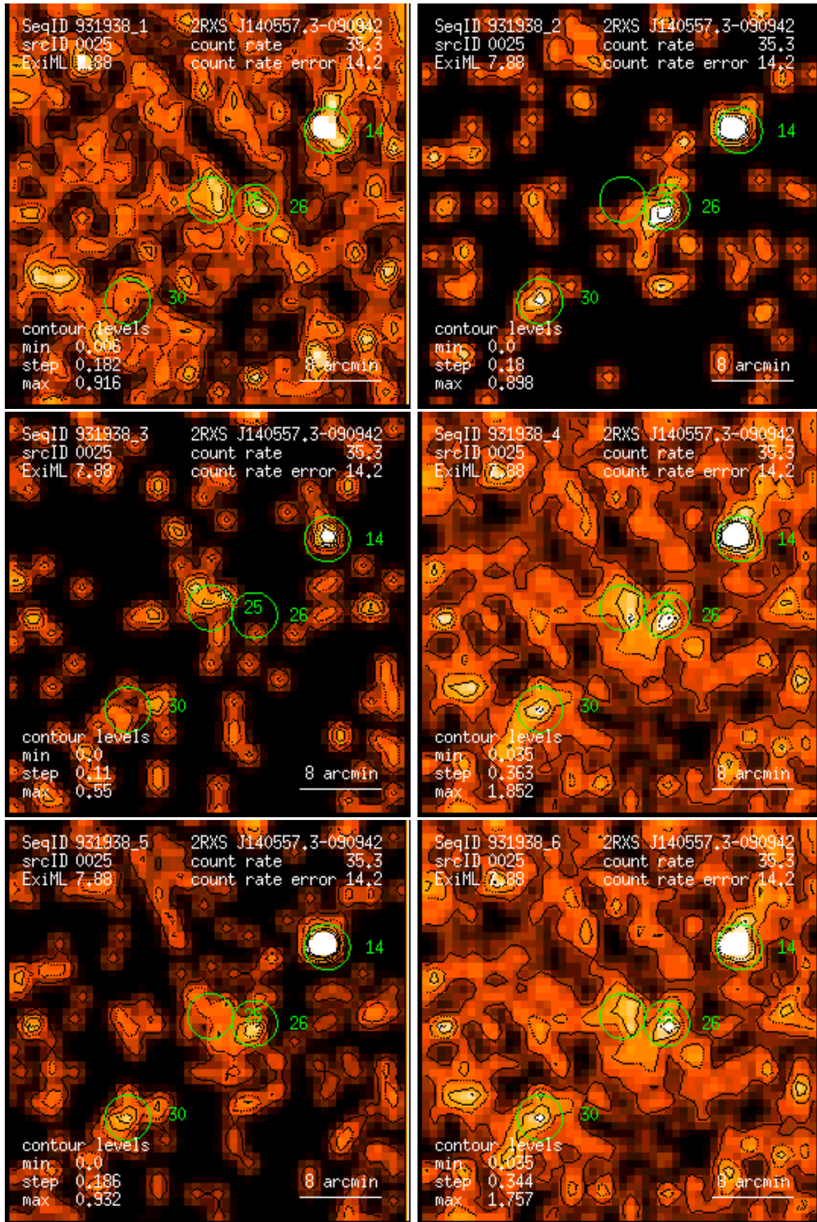
Figure 25: RASS 931938: detection 0025: band rate images, Gaussian filter: (1) PSPC channels 11 – 41, (2) 52 – 90, (3) 91 – 201, (4) 11 – 235, (5) 52 – 201, (6) 11 – 201. Broad band rates in counts/ks. Band rate contour levels in counts/ks/arcmin 2 .
