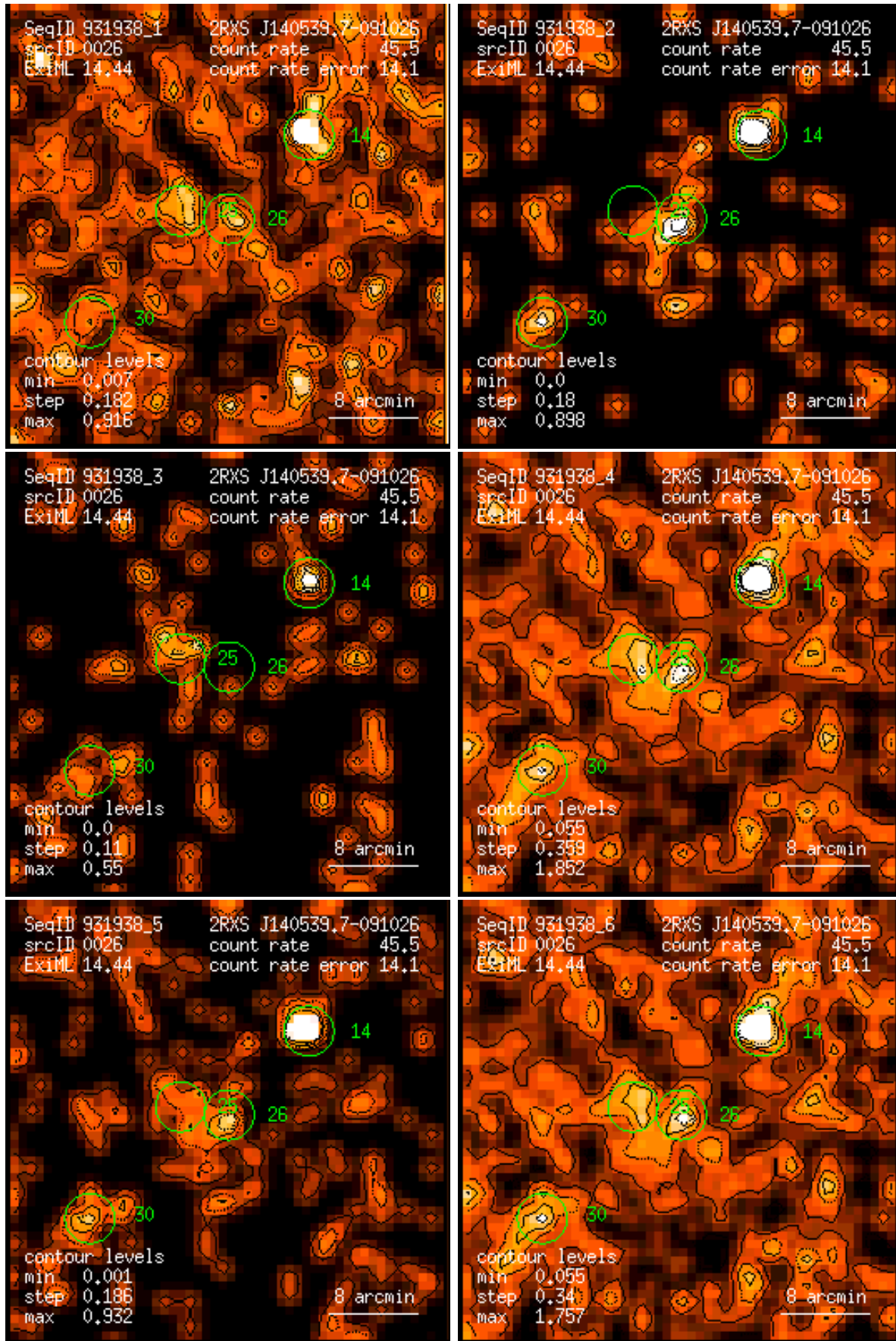
Figure 26: RASS 931938: detection 0026: band rate images, Gaussian filter: (1) PSPC channels 11 – 41, (2) 52 – 90, (3) 91 – 201, (4) 11 – 235, (5) 52 – 201, (6) 11 – 201. Broad band rates in counts/ks. Band rate contour levels in counts/ks/arcmin 2 .
