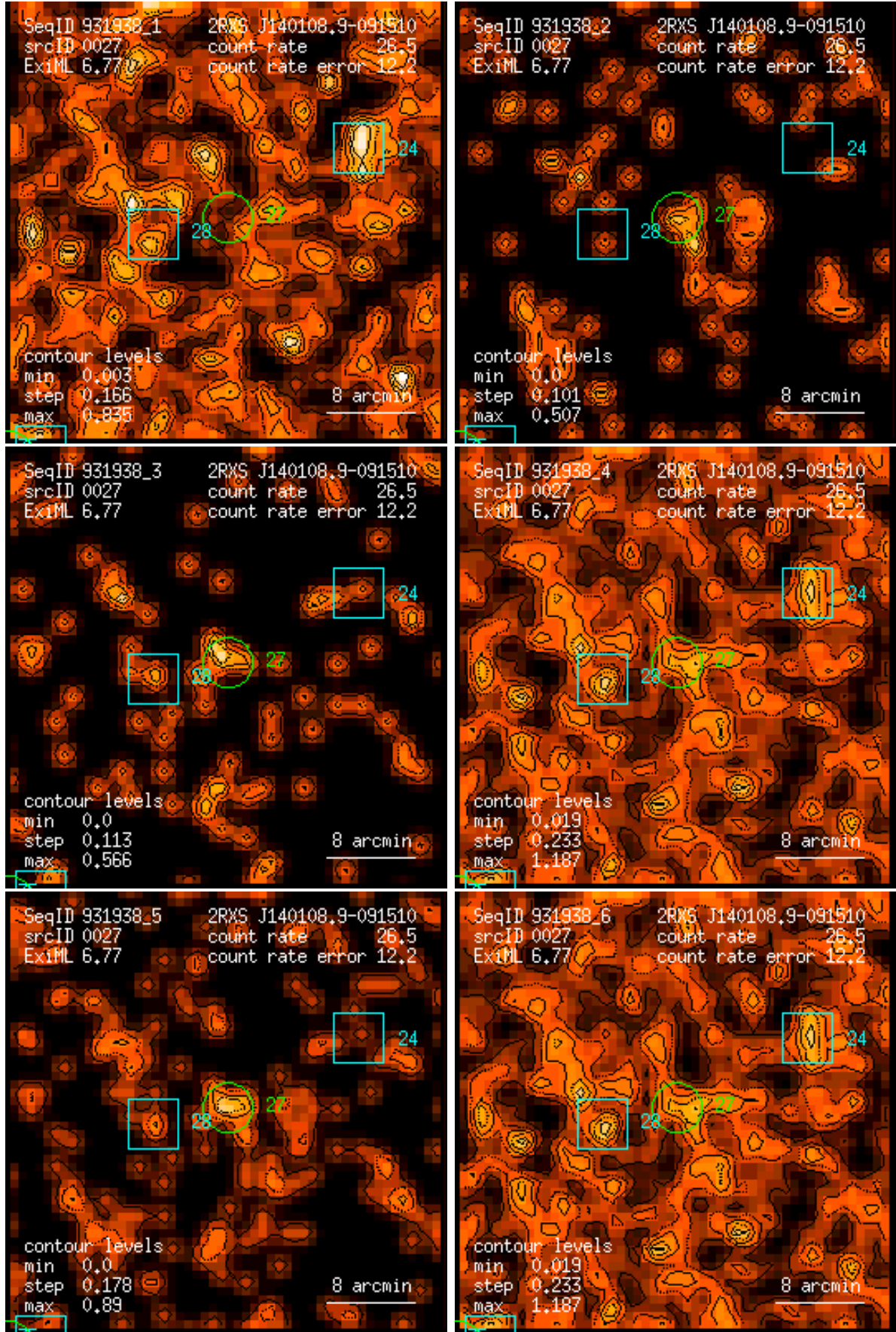
Figure 27: RASS 931938: detection 0027: band rate images, Gaussian filter: (1) PSPC channels 11 – 41, (2) 52 – 90, (3) 91 – 201, (4) 11 – 235, (5) 52 – 201, (6) 11 – 201. Broad band rates in counts/ks. Band rate contour levels in counts/ks/arcmin 2 .
