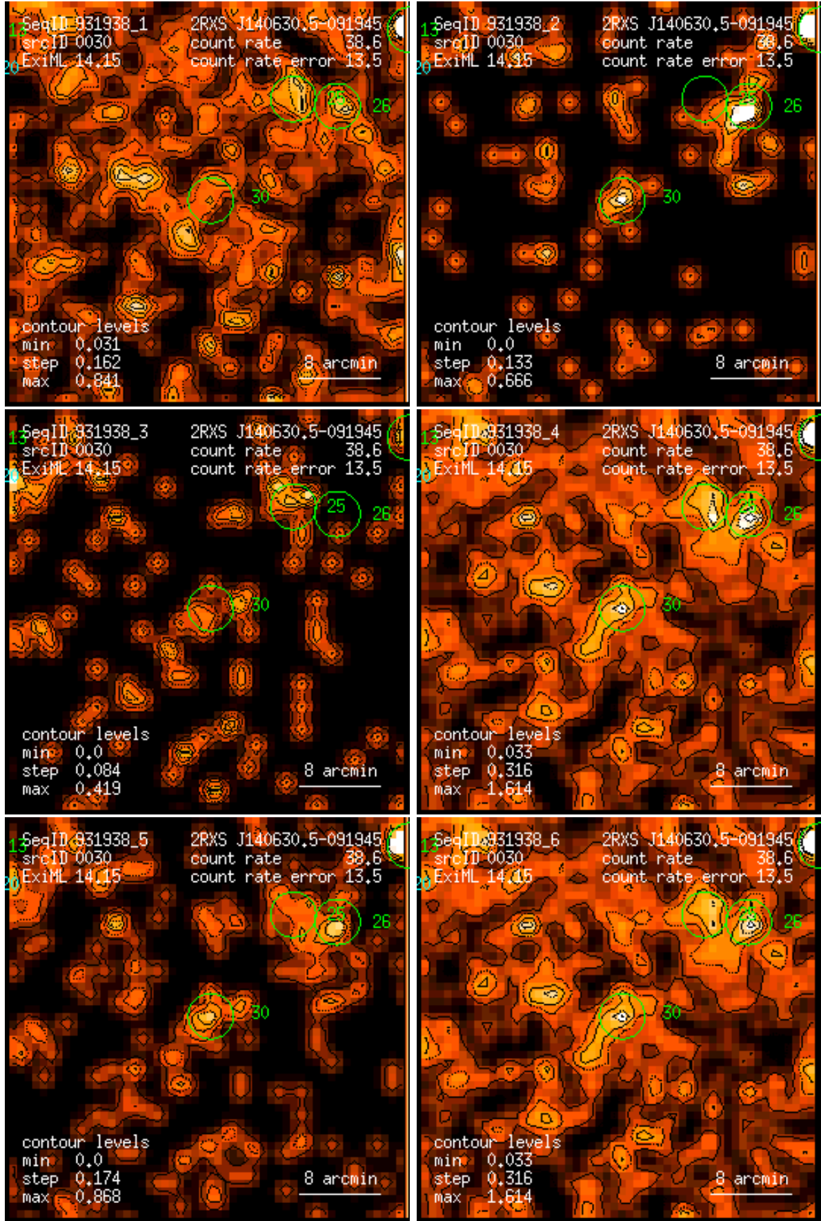
Figure 30: RASS 931938: detection 0030: band rate images, Gaussian filter: (1) PSPC channels 11 – 41, (2) 52 – 90, (3) 91 – 201, (4) 11 – 235, (5) 52 – 201, (6) 11 – 201. Broad band rates in counts/ks. Band rate contour levels in counts/ks/arcmin 2 .
