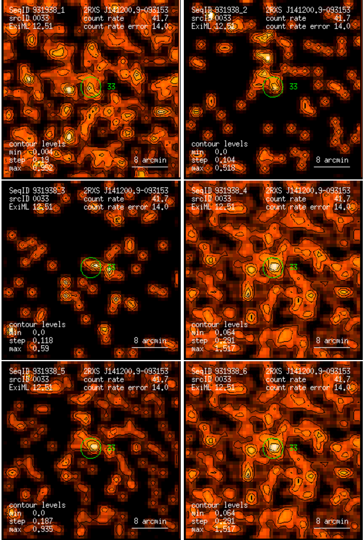
Figure 33: RASS 931938: detection 0033: band rate images, Gaussian filter: (1) PSPC channels 11 – 41, (2) 52 – 90, (3) 91 – 201, (4) 11 – 235, (5) 52 – 201, (6) 11 – 201. Broad band rates in counts/ks. Band rate contour levels in counts/ks/arcmin 2 .
