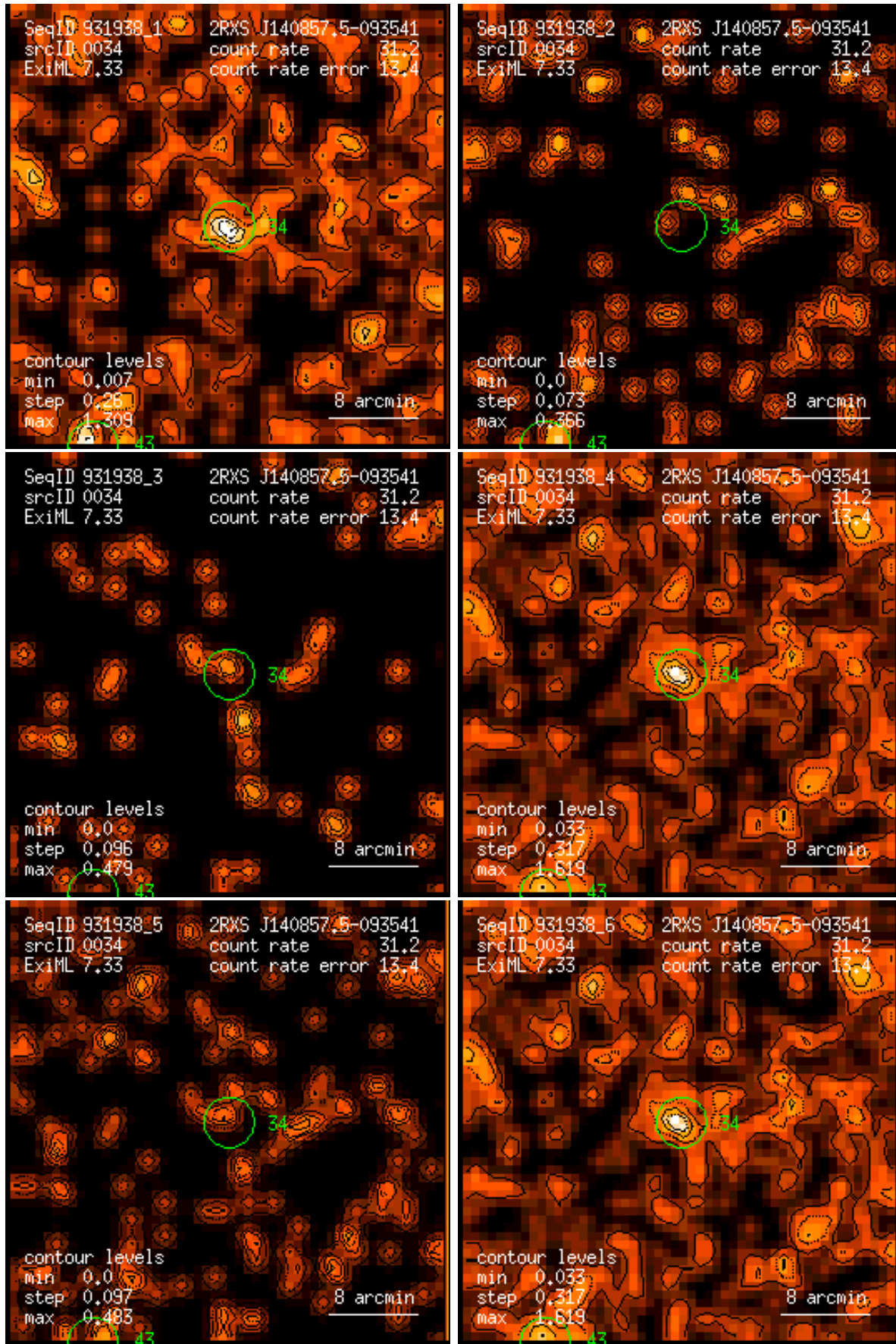
Figure 34: RASS 931938: detection 0034: band rate images, Gaussian filter: (1) PSPC channels 11 – 41, (2) 52 – 90, (3) 91 – 201, (4) 11 – 235, (5) 52 – 201, (6) 11 – 201. Broad band rates in counts/ks. Band rate contour levels in counts/ks/arcmin 2 .
