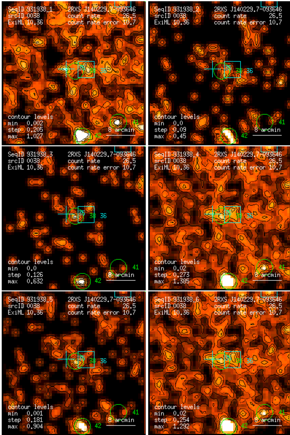
Figure 38: RASS 931938: detection 0038: band rate images, Gaussian filter: (1) PSPC channels 11 – 41, (2) 52 – 90, (3) 91 – 201, (4) 11 – 235, (5) 52 – 201, (6) 11 – 201. Broad band rates in counts/ks. Band rate contour levels in counts/ks/arcmin 2 .
