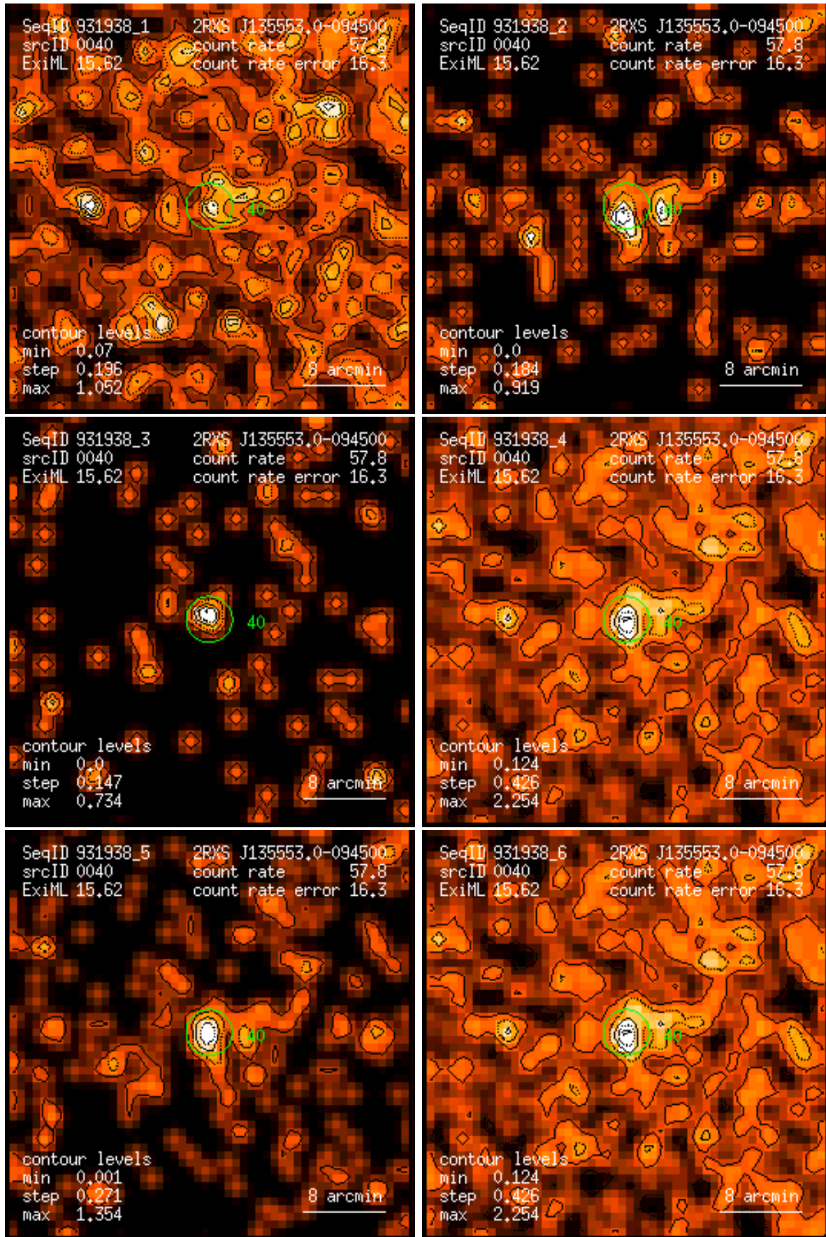
Figure 40: RASS 931938: detection 0040: band rate images, Gaussian filter: (1) PSPC channels 11 – 41, (2) 52 – 90, (3) 91 – 201, (4) 11 – 235, (5) 52 – 201, (6) 11 – 201. Broad band rates in counts/ks. Band rate contour levels in counts/ks/arcmin 2 .
