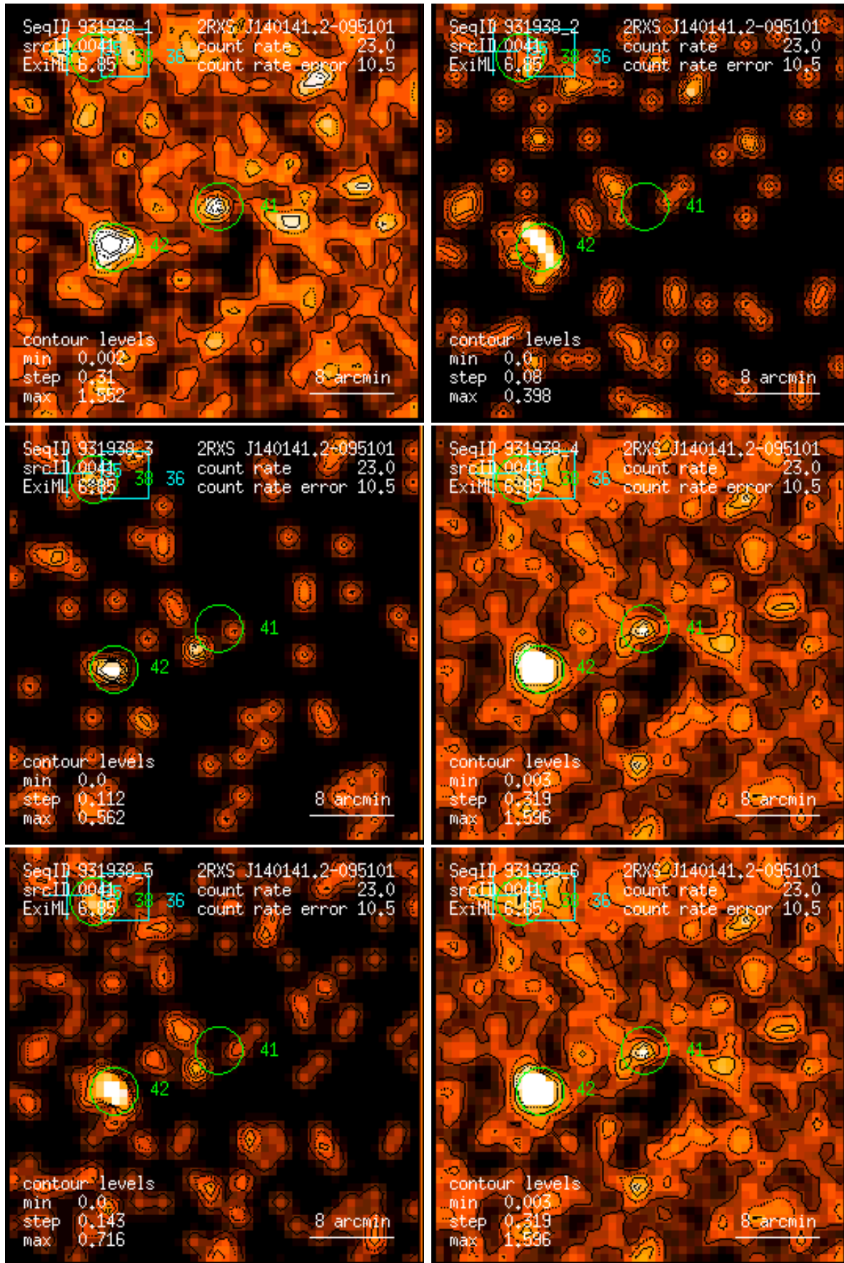
Figure 41: RASS 931938: detection 0041: band rate images, Gaussian filter: (1) PSPC channels 11 – 41, (2) 52 – 90, (3) 91 – 201, (4) 11 – 235, (5) 52 – 201, (6) 11 – 201. Broad band rates in counts/ks. Band rate contour levels in counts/ks/arcmin 2 .
