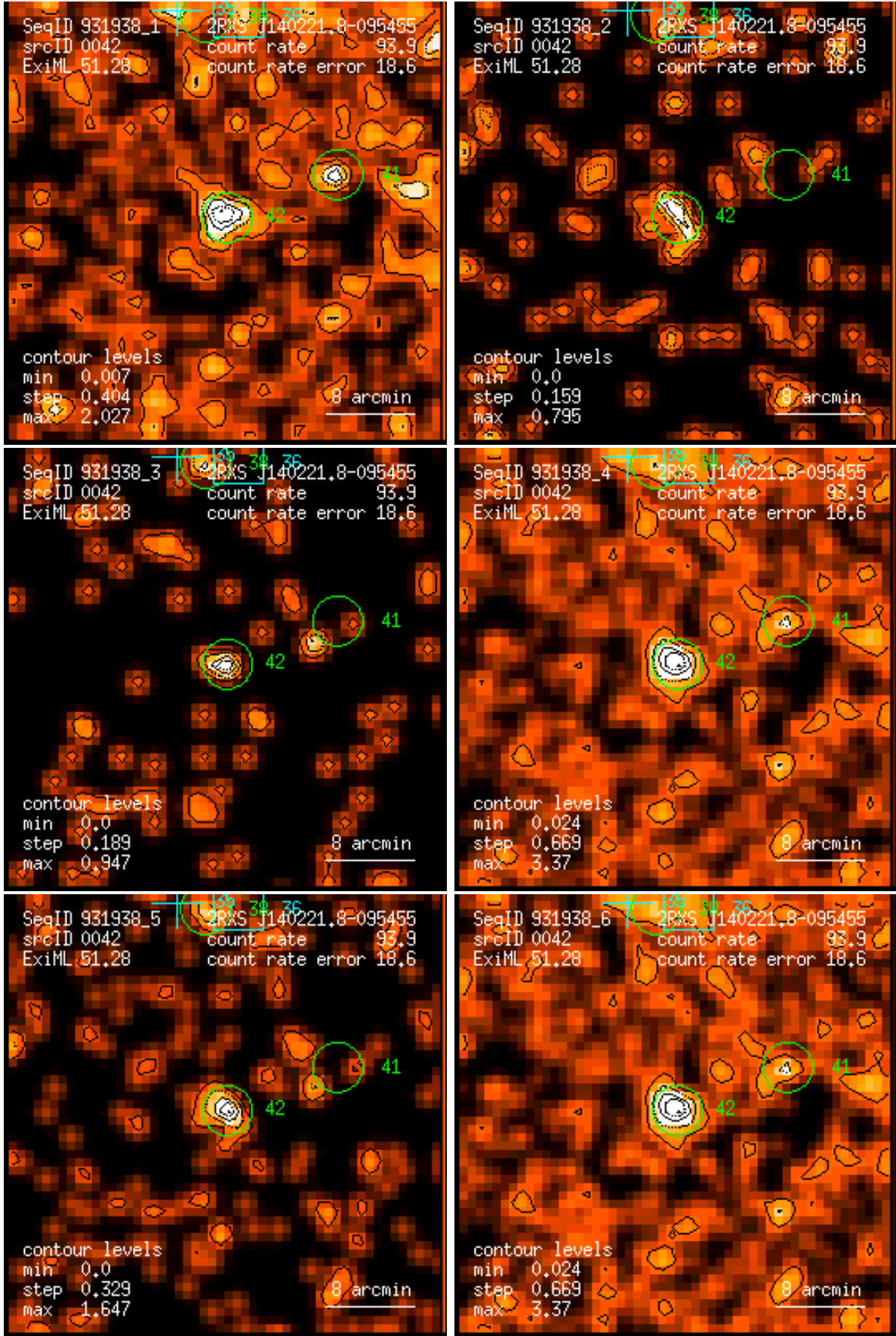
Figure 42: RASS 931938: detection 0042: band rate images, Gaussian filter: (1) PSPC channels 11 – 41, (2) 52 – 90, (3) 91 – 201, (4) 11 – 235, (5) 52 – 201, (6) 11 – 201. Broad band rates in counts/ks. Band rate contour levels in counts/ks/arcmin 2 .
