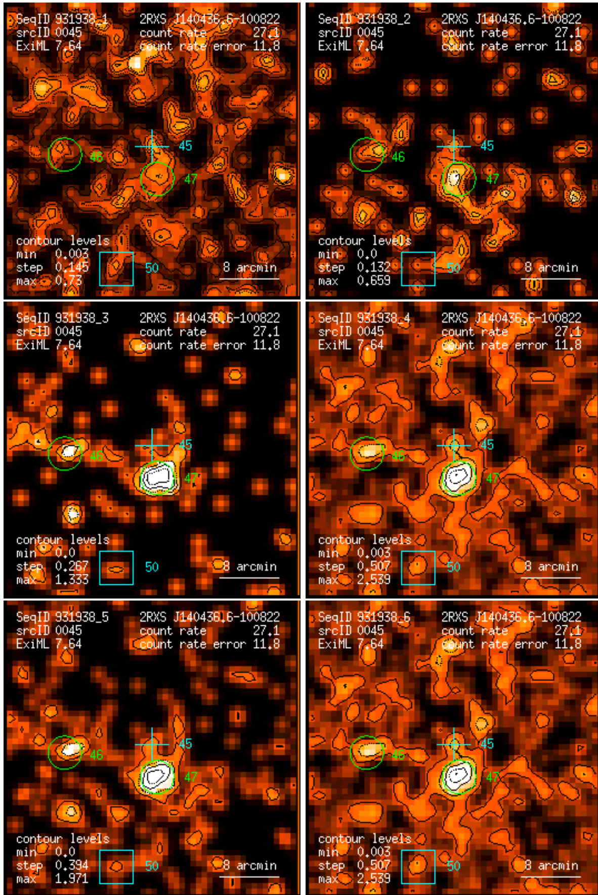
Figure 45: RASS 931938: detection 0045: band rate images, Gaussian filter: (1) PSPC channels 11 – 41, (2) 52 – 90, (3) 91 – 201, (4) 11 – 235, (5) 52 – 201, (6) 11 – 201. Broad band rates in counts/ks. Band rate contour levels in counts/ks/arcmin 2 .
