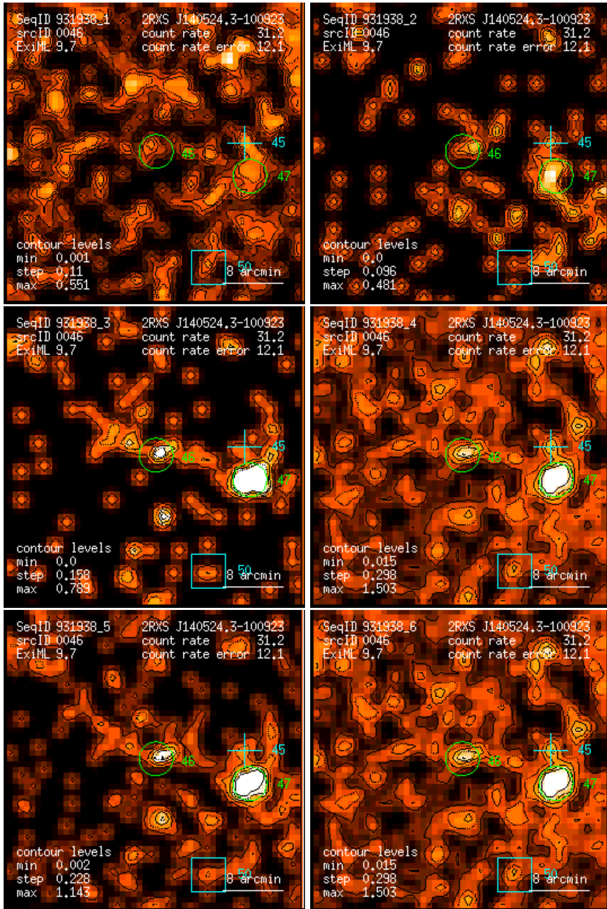
Figure 46: RASS 931938: detection 0046: band rate images, Gaussian filter: (1) PSPC channels 11 – 41, (2) 52 – 90, (3) 91 – 201, (4) 11 – 235, (5) 52 – 201, (6) 11 – 201. Broad band rates in counts/ks. Band rate contour levels in counts/ks/arcmin 2 .
