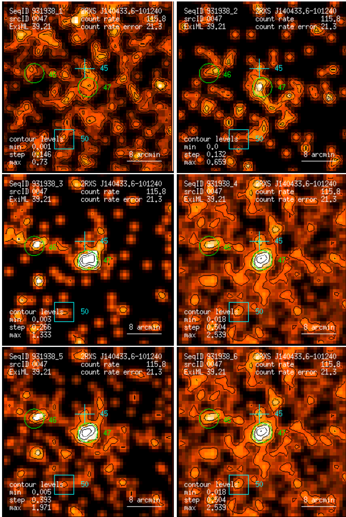
Figure 47: RASS 931938: detection 0047: band rate images, Gaussian filter: (1) PSPC channels 11 – 41, (2) 52 – 90, (3) 91 – 201, (4) 11 – 235, (5) 52 – 201, (6) 11 – 201. Broad band rates in counts/ks. Band rate contour levels in counts/ks/arcmin 2 .
