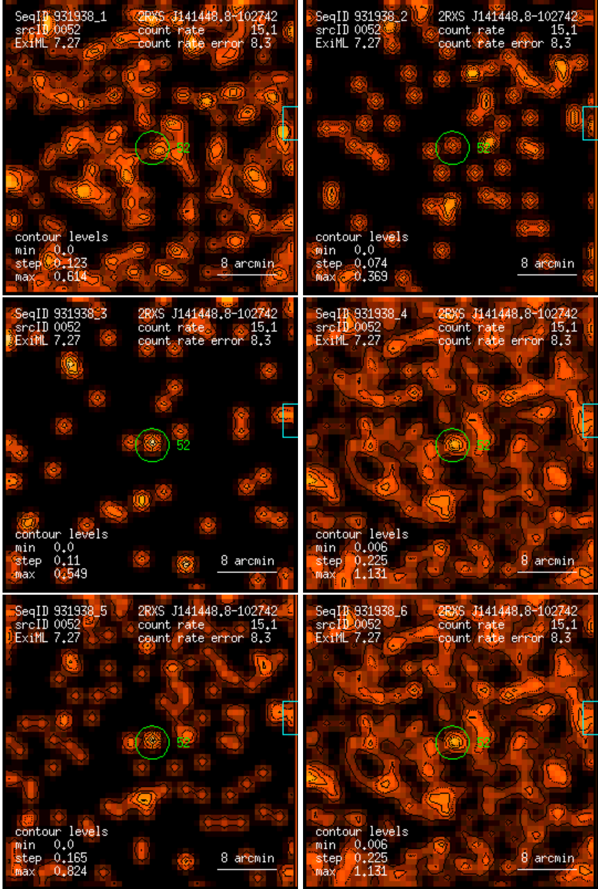
Figure 52: RASS 931938: detection 0052: band rate images, Gaussian filter: (1) PSPC channels 11 – 41, (2) 52 – 90, (3) 91 – 201, (4) 11 – 235, (5) 52 – 201, (6) 11 – 201. Broad band rates in counts/ks. Band rate contour levels in counts/ks/arcmin 2 .
