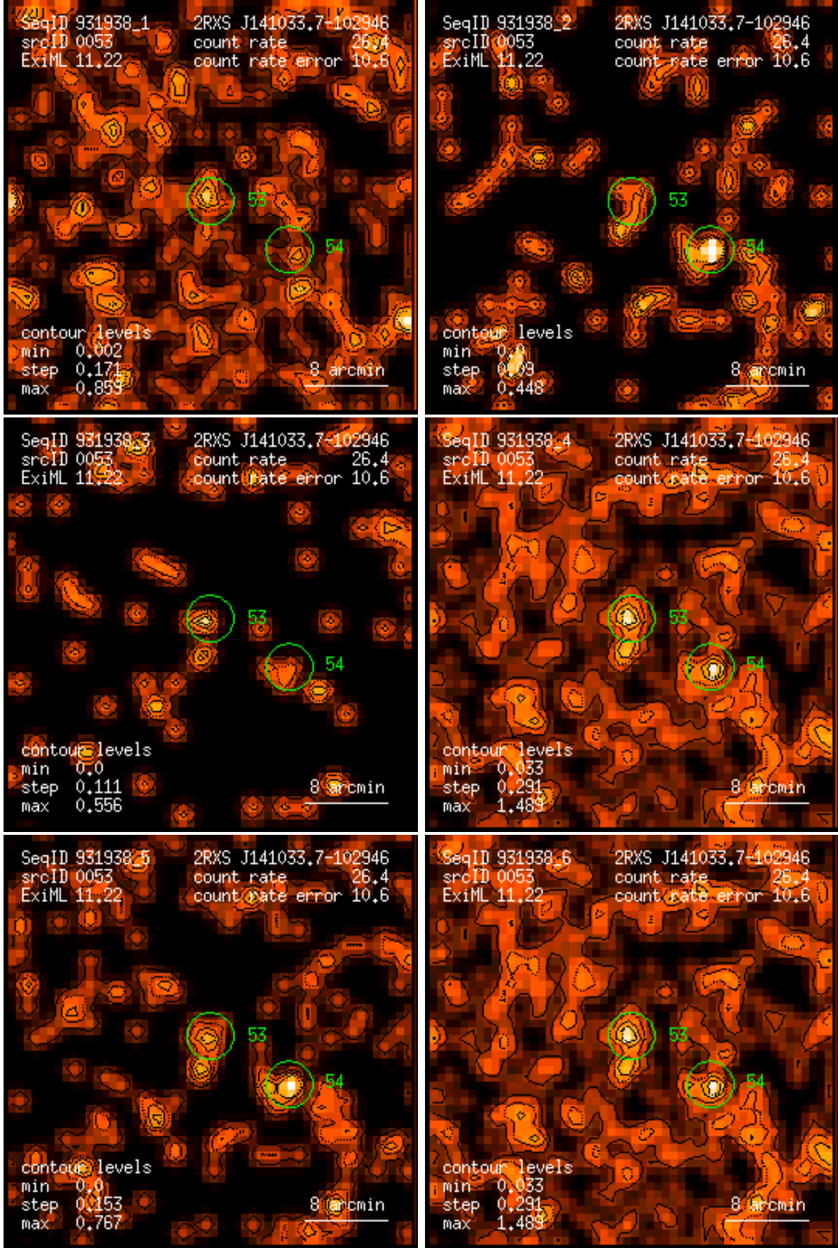
Figure 53: RASS 931938: detection 0053: band rate images, Gaussian filter: (1) PSPC channels 11 – 41, (2) 52 – 90, (3) 91 – 201, (4) 11 – 235, (5) 52 – 201, (6) 11 – 201. Broad band rates in counts/ks. Band rate contour levels in counts/ks/arcmin 2 .
