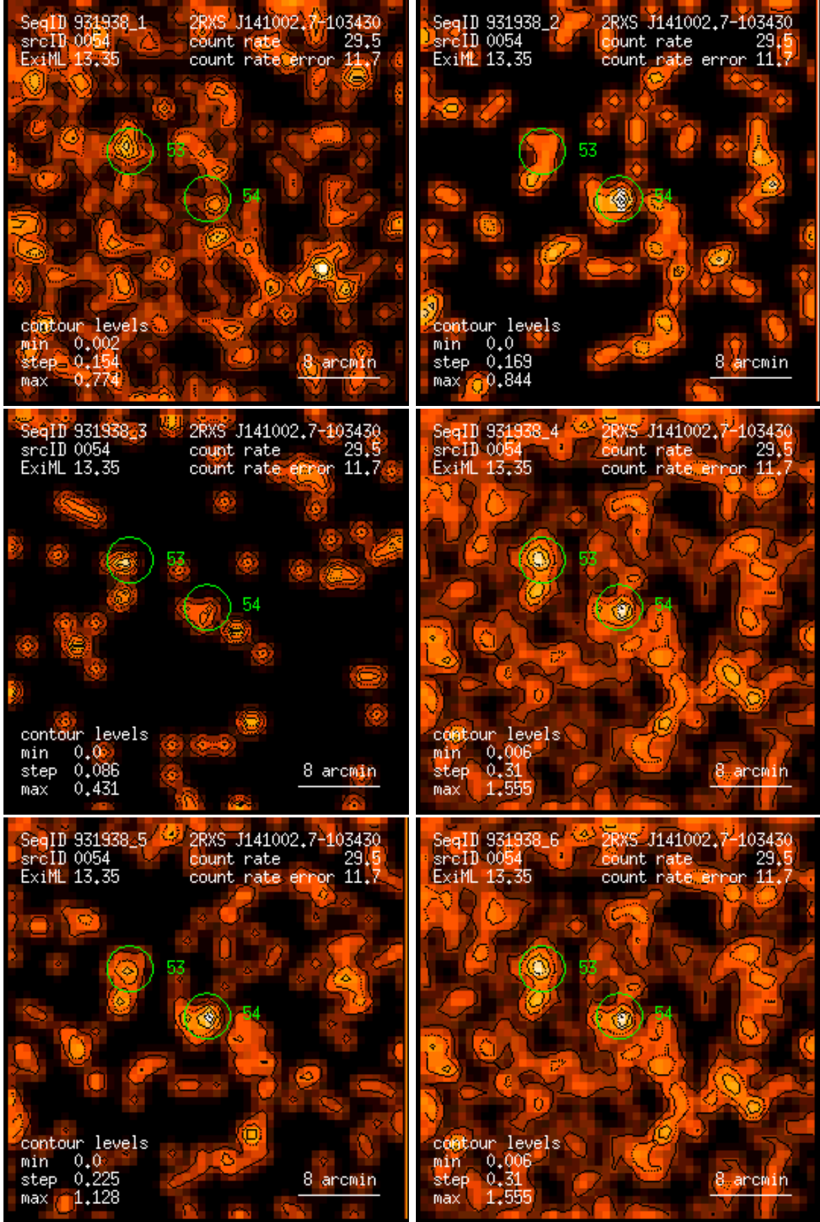
Figure 54: RASS 931938: detection 0054: band rate images, Gaussian filter: (1) PSPC channels 11 – 41, (2) 52 – 90, (3) 91 – 201, (4) 11 – 235, (5) 52 – 201, (6) 11 – 201. Broad band rates in counts/ks. Band rate contour levels in counts/ks/arcmin 2 .
