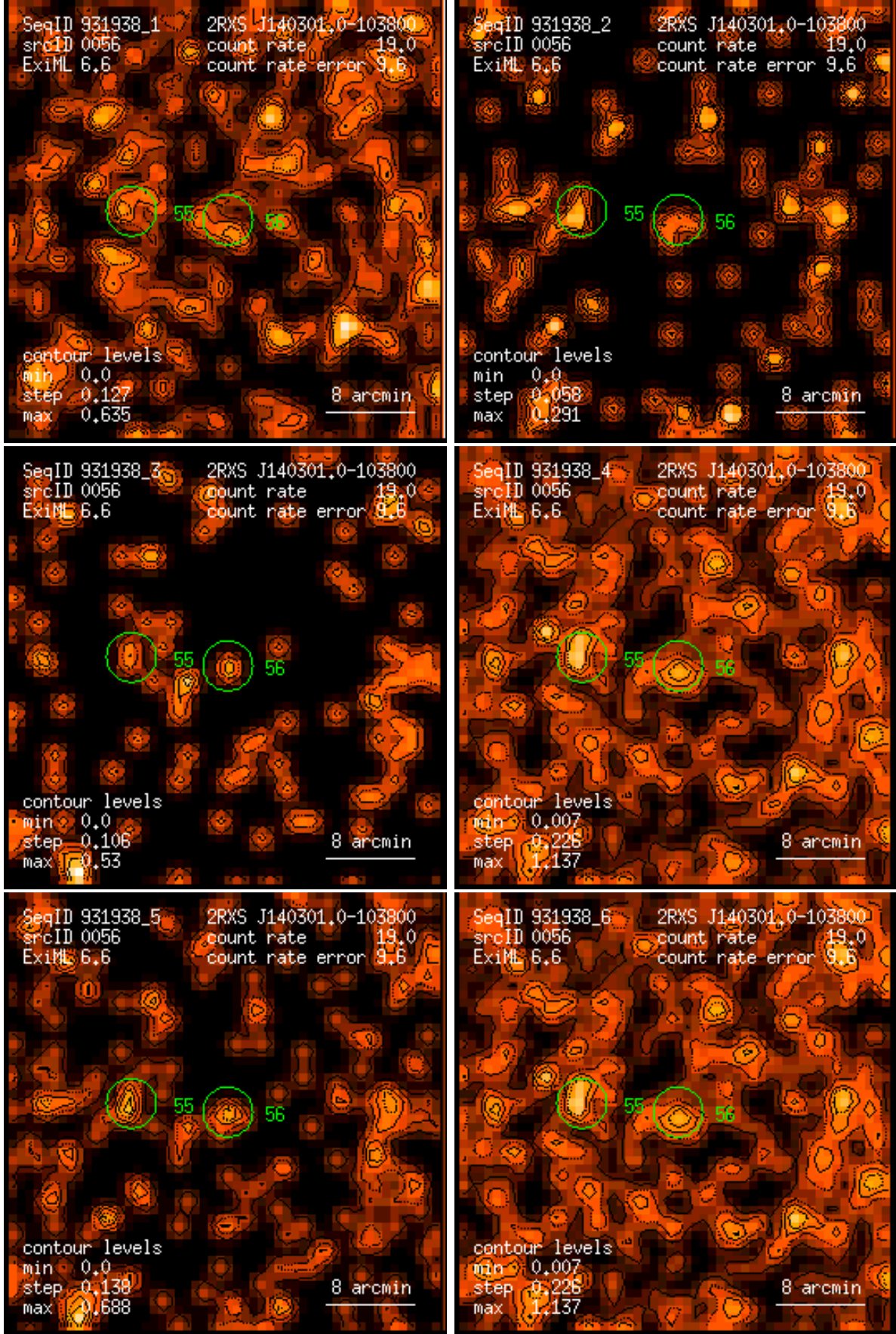
Figure 56: RASS 931938: detection 0056: band rate images, Gaussian filter: (1) PSPC channels 11 – 41, (2) 52 – 90, (3) 91 – 201, (4) 11 – 235, (5) 52 – 201, (6) 11 – 201. Broad band rates in counts/ks. Band rate contour levels in counts/ks/arcmin 2 .
