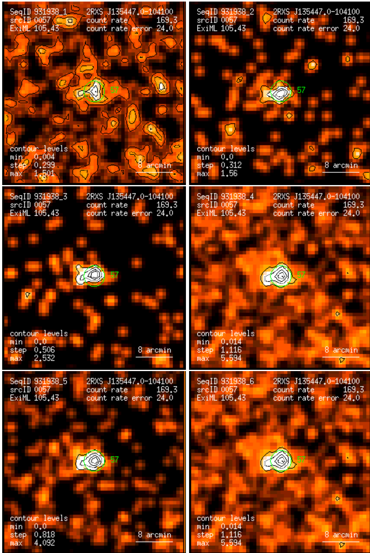
Figure 57: RASS 931938: detection 0057: band rate images, Gaussian filter: (1) PSPC channels 11 – 41, (2) 52 – 90, (3) 91 – 201, (4) 11 – 235, (5) 52 – 201, (6) 11 – 201. Broad band rates in counts/ks. Band rate contour levels in counts/ks/arcmin 2 .
