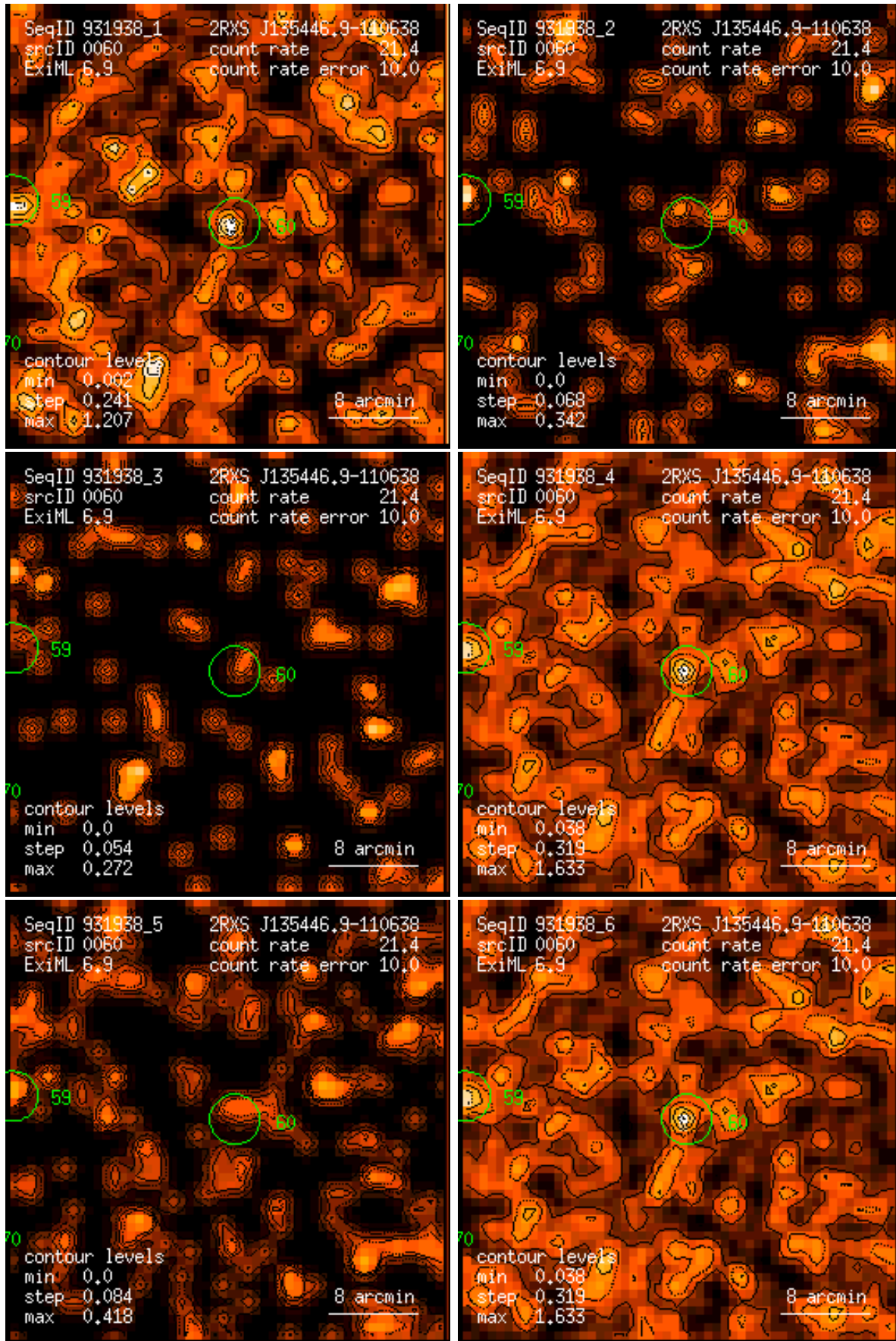
Figure 60: RASS 931938: detection 0060: band rate images, Gaussian filter: (1) PSPC channels 11 – 41, (2) 52 – 90, (3) 91 – 201, (4) 11 – 235, (5) 52 – 201, (6) 11 – 201. Broad band rates in counts/ks. Band rate contour levels in counts/ks/arcmin 2 .
