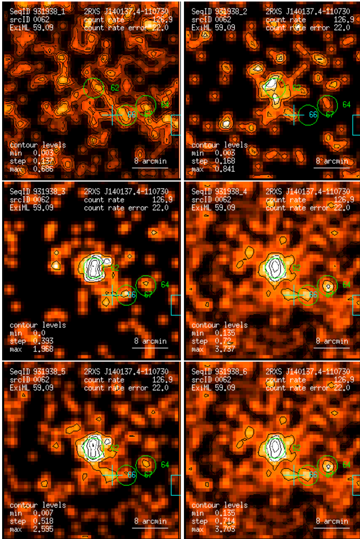
Figure 62: RASS 931938: detection 0062: band rate images, Gaussian filter: (1) PSPC channels 11 – 41, (2) 52 – 90, (3) 91 – 201, (4) 11 – 235, (5) 52 – 201, (6) 11 – 201. Broad band rates in counts/ks. Band rate contour levels in counts/ks/arcmin 2 .
