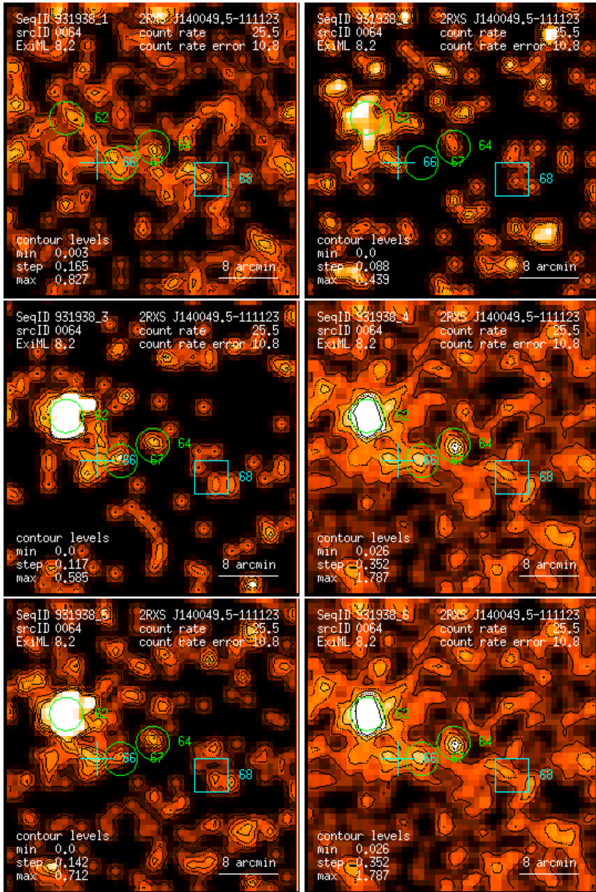
Figure 64: RASS 931938: detection 0064: band rate images, Gaussian filter: (1) PSPC channels 11 – 41, (2) 52 – 90, (3) 91 – 201, (4) 11 – 235, (5) 52 – 201, (6) 11 – 201. Broad band rates in counts/ks. Band rate contour levels in counts/ks/arcmin 2 .
