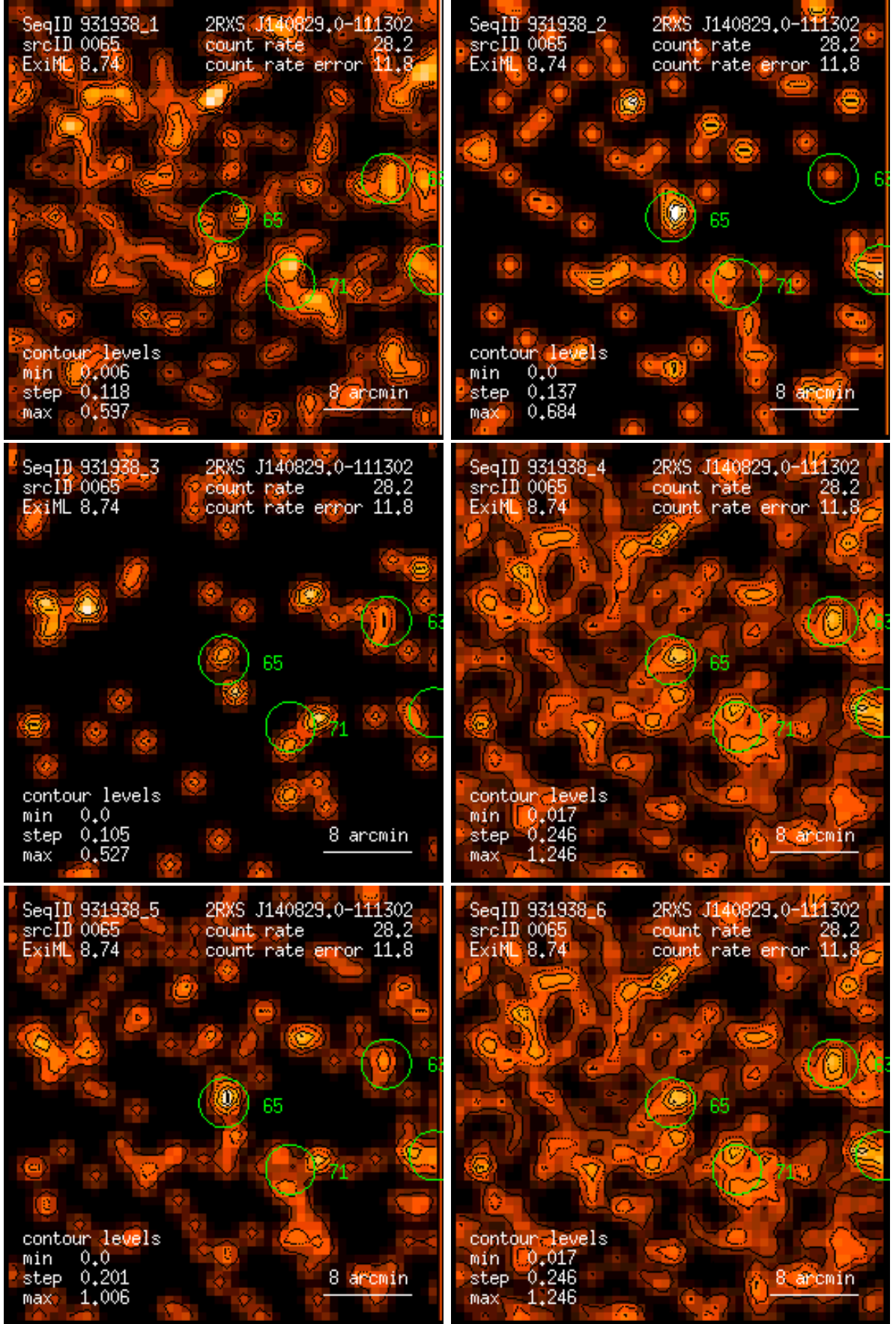
Figure 65: RASS 931938: detection 0065: band rate images, Gaussian filter: (1) PSPC channels 11 – 41, (2) 52 – 90, (3) 91 – 201, (4) 11 – 235, (5) 52 – 201, (6) 11 – 201. Broad band rates in counts/ks. Band rate contour levels in counts/ks/arcmin 2 .
