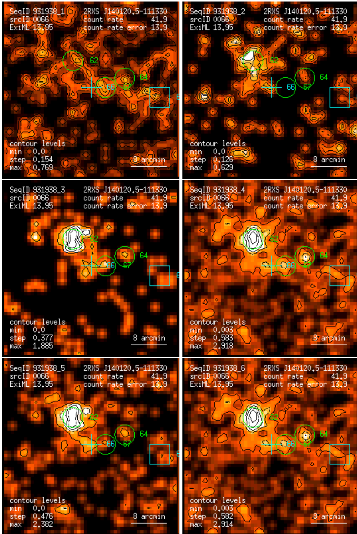
Figure 66: RASS 931938: detection 0066: band rate images, Gaussian filter: (1) PSPC channels 11 – 41, (2) 52 – 90, (3) 91 – 201, (4) 11 – 235, (5) 52 – 201, (6) 11 – 201. Broad band rates in counts/ks. Band rate contour levels in counts/ks/arcmin 2 .
