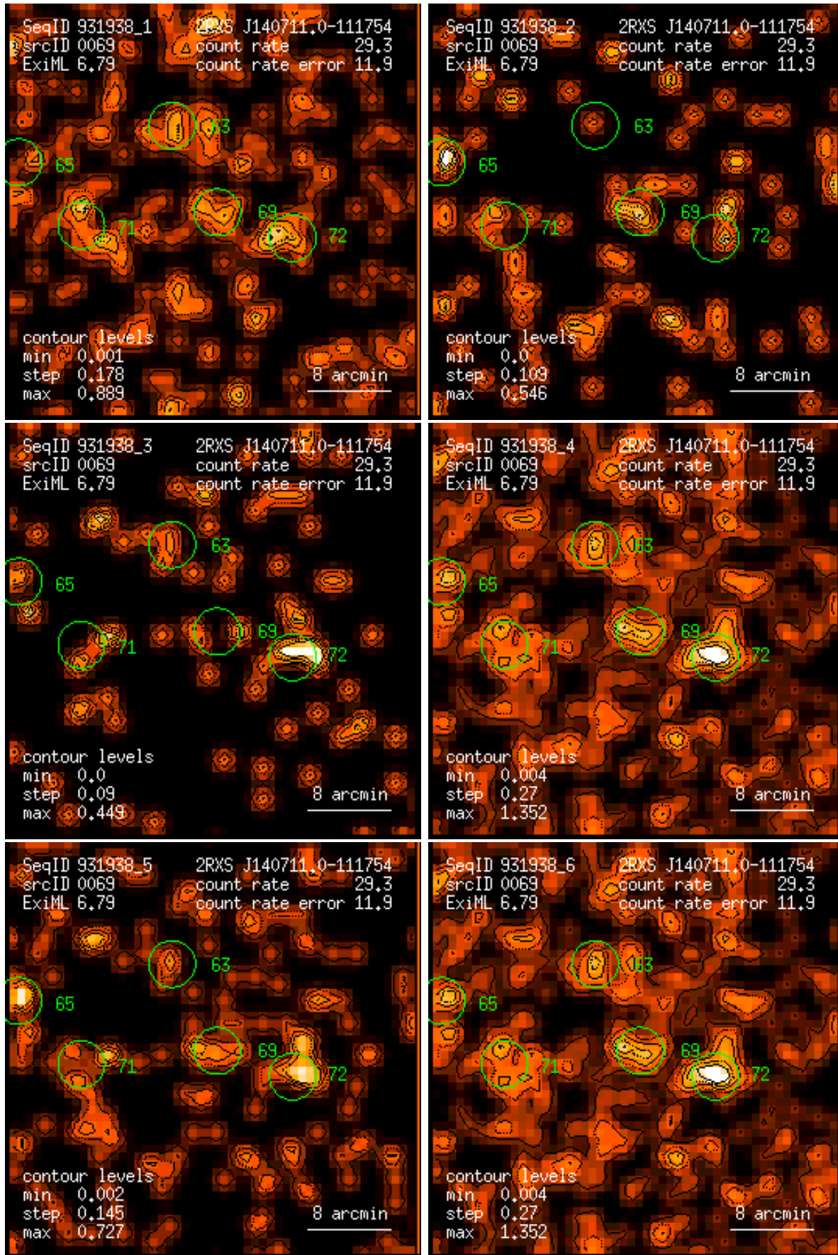
Figure 69: RASS 931938: detection 0069: band rate images, Gaussian filter: (1) PSPC channels 11 – 41, (2) 52 – 90, (3) 91 – 201, (4) 11 – 235, (5) 52 – 201, (6) 11 – 201. Broad band rates in counts/ks. Band rate contour levels in counts/ks/arcmin 2 .
