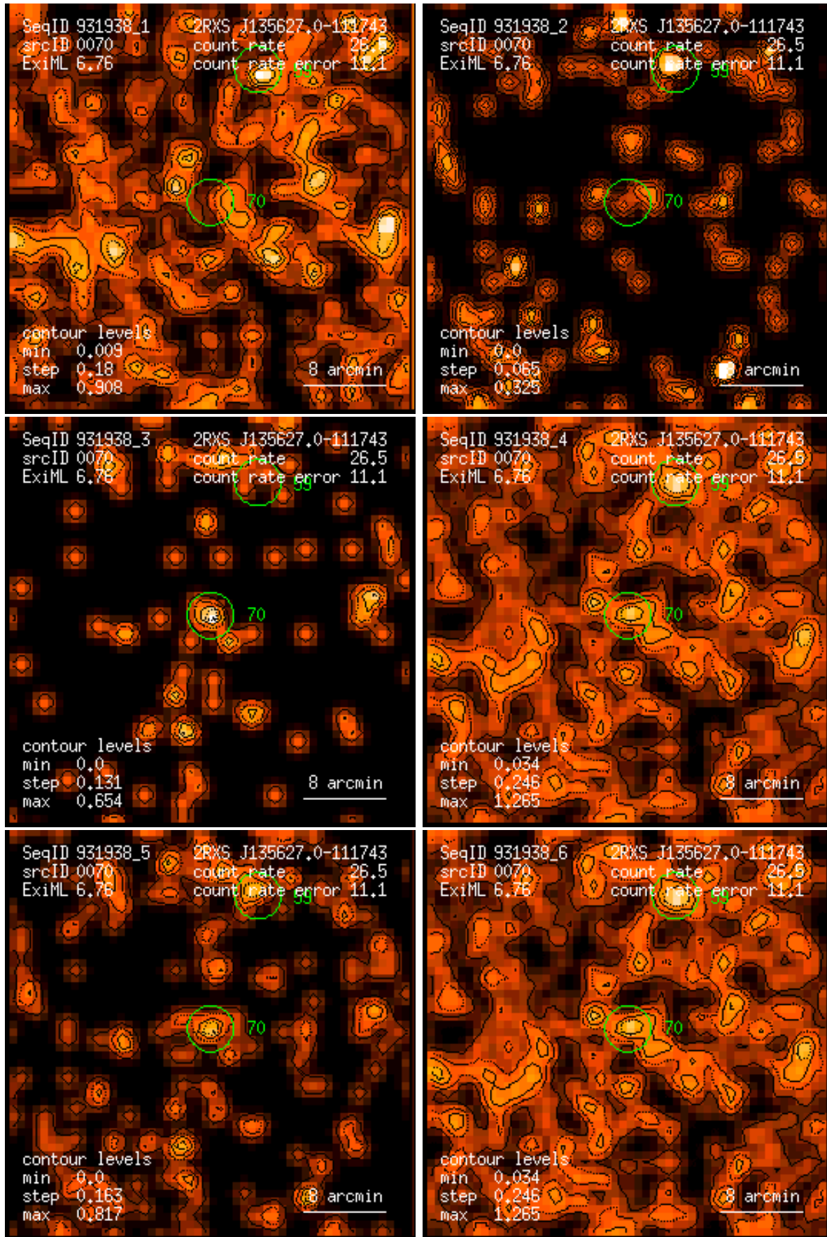
Figure 70: RASS 931938: detection 0070: band rate images, Gaussian filter: (1) PSPC channels 11 – 41, (2) 52 – 90, (3) 91 – 201, (4) 11 – 235, (5) 52 – 201, (6) 11 – 201. Broad band rates in counts/ks. Band rate contour levels in counts/ks/arcmin 2 .
