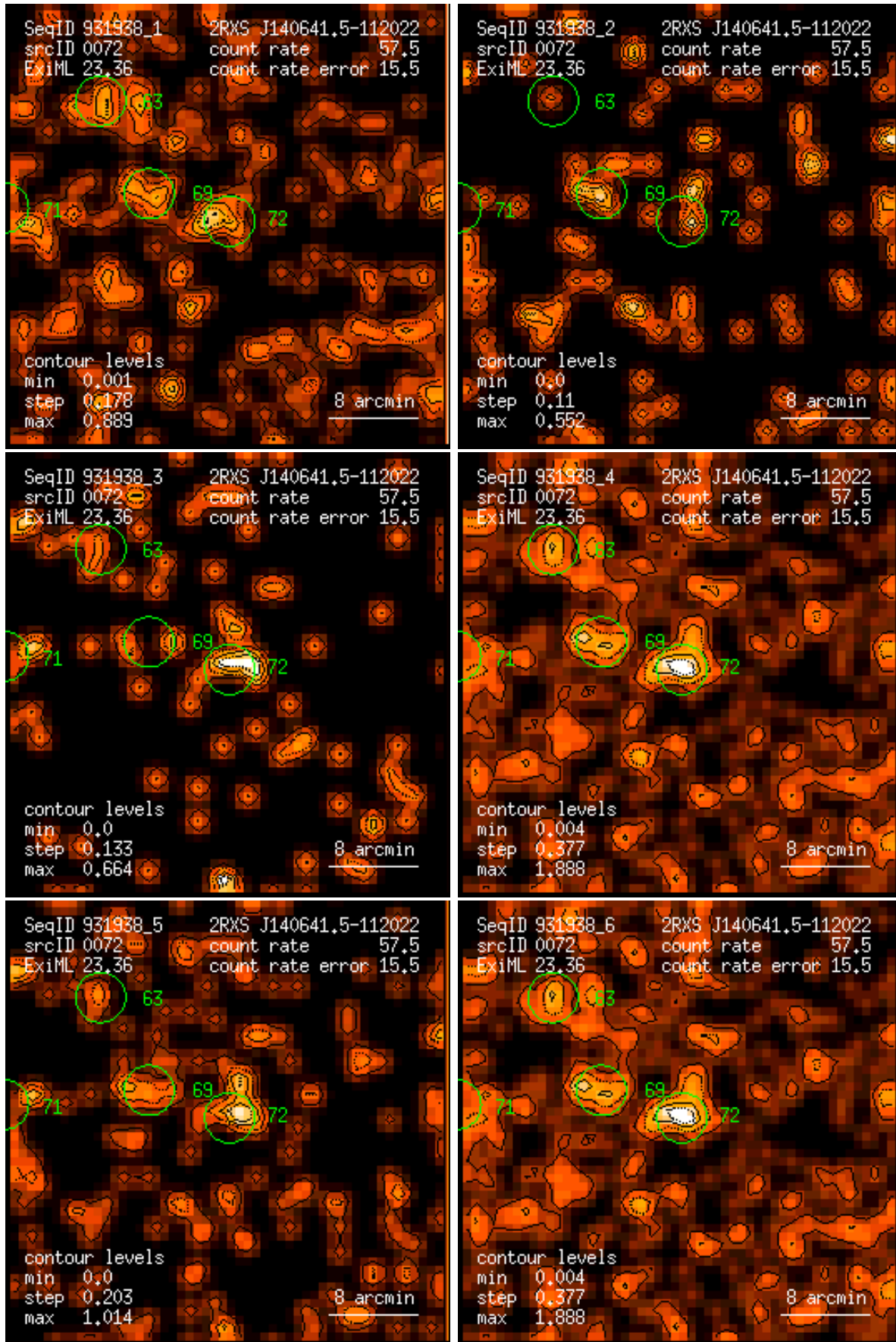
Figure 72: RASS 931938: detection 0072: band rate images, Gaussian filter: (1) PSPC channels 11 – 41, (2) 52 – 90, (3) 91 – 201, (4) 11 – 235, (5) 52 – 201, (6) 11 – 201. Broad band rates in counts/ks. Band rate contour levels in counts/ks/arcmin 2 .
