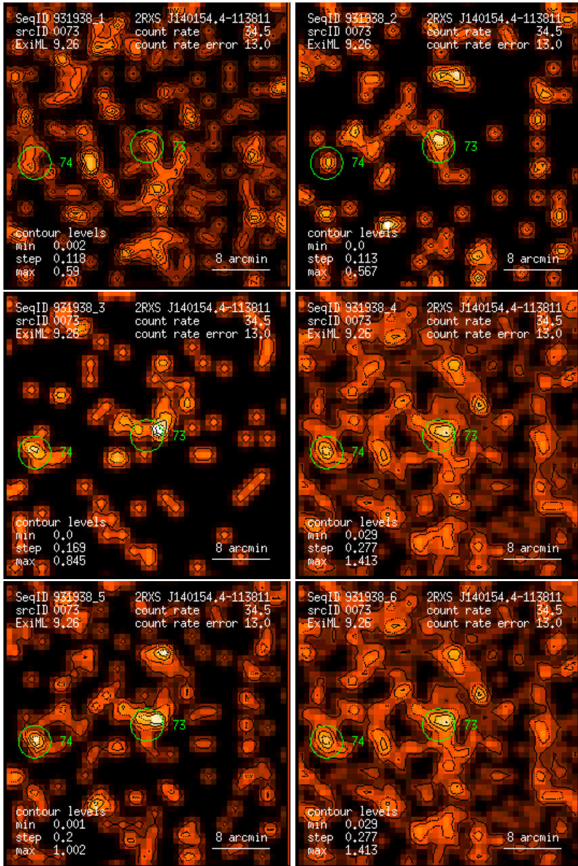
Figure 73: RASS 931938: detection 0073: band rate images, Gaussian filter: (1) PSPC channels 11 – 41, (2) 52 – 90, (3) 91 – 201, (4) 11 – 235, (5) 52 – 201, (6) 11 – 201. Broad band rates in counts/ks. Band rate contour levels in counts/ks/arcmin 2 .
