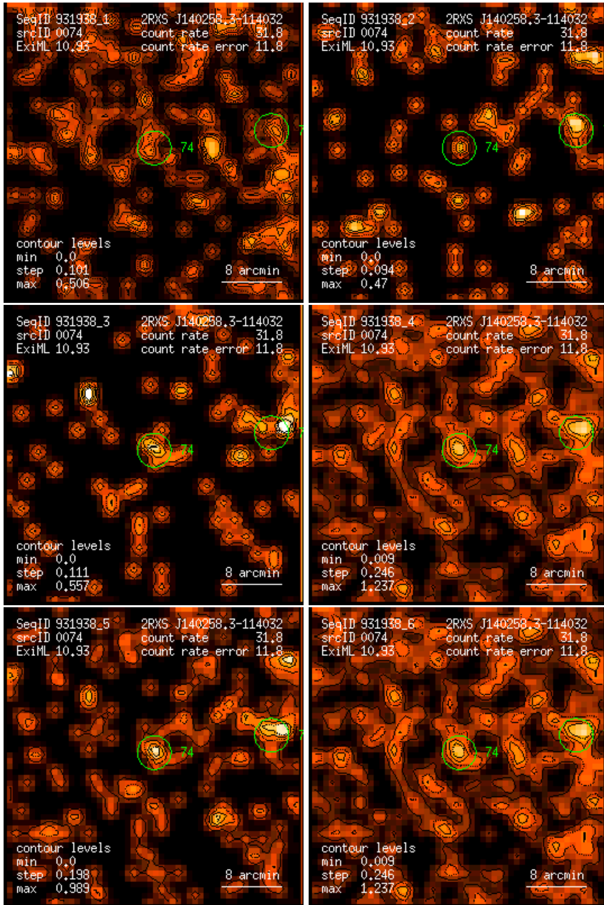
Figure 74: RASS 931938: detection 0074: band rate images, Gaussian filter: (1) PSPC channels 11 – 41, (2) 52 – 90, (3) 91 – 201, (4) 11 – 235, (5) 52 – 201, (6) 11 – 201. Broad band rates in counts/ks. Band rate contour levels in counts/ks/arcmin 2 .
