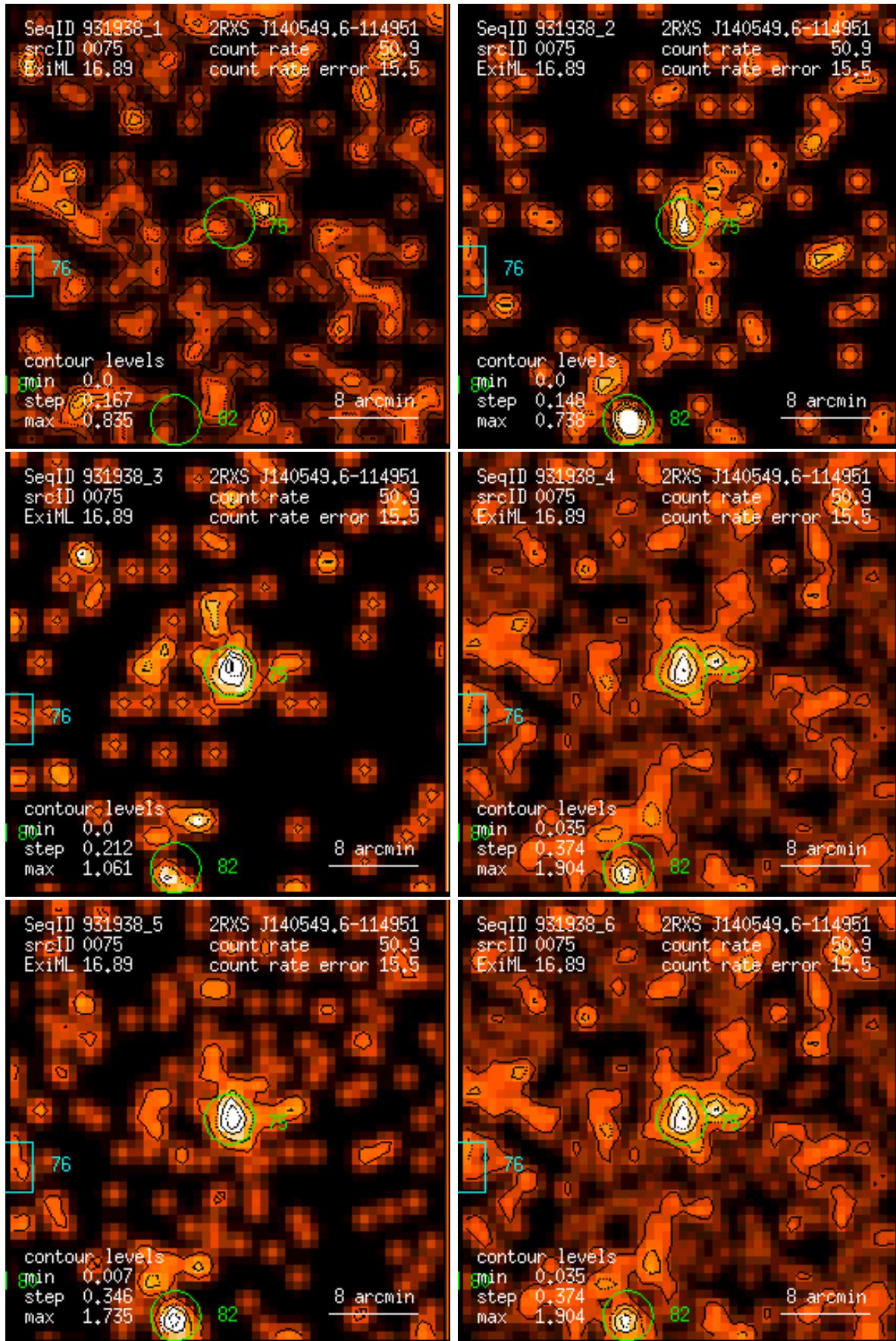
Figure 75: RASS 931938: detection 0075: band rate images, Gaussian filter: (1) PSPC channels 11 – 41, (2) 52 – 90, (3) 91 – 201, (4) 11 – 235, (5) 52 – 201, (6) 11 – 201. Broad band rates in counts/ks. Band rate contour levels in counts/ks/arcmin 2 .
