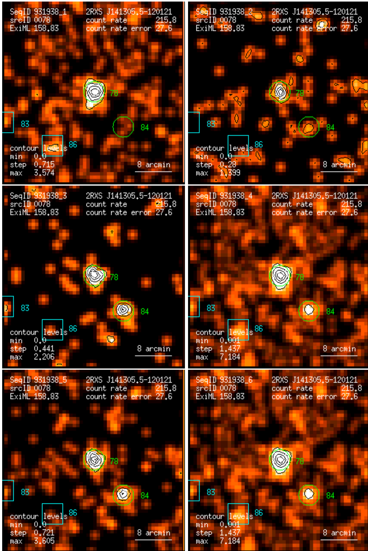
Figure 78: RASS 931938: detection 0078: band rate images, Gaussian filter: (1) PSPC channels 11 – 41, (2) 52 – 90, (3) 91 – 201, (4) 11 – 235, (5) 52 – 201, (6) 11 – 201. Broad band rates in counts/ks. Band rate contour levels in counts/ks/arcmin 2 .
