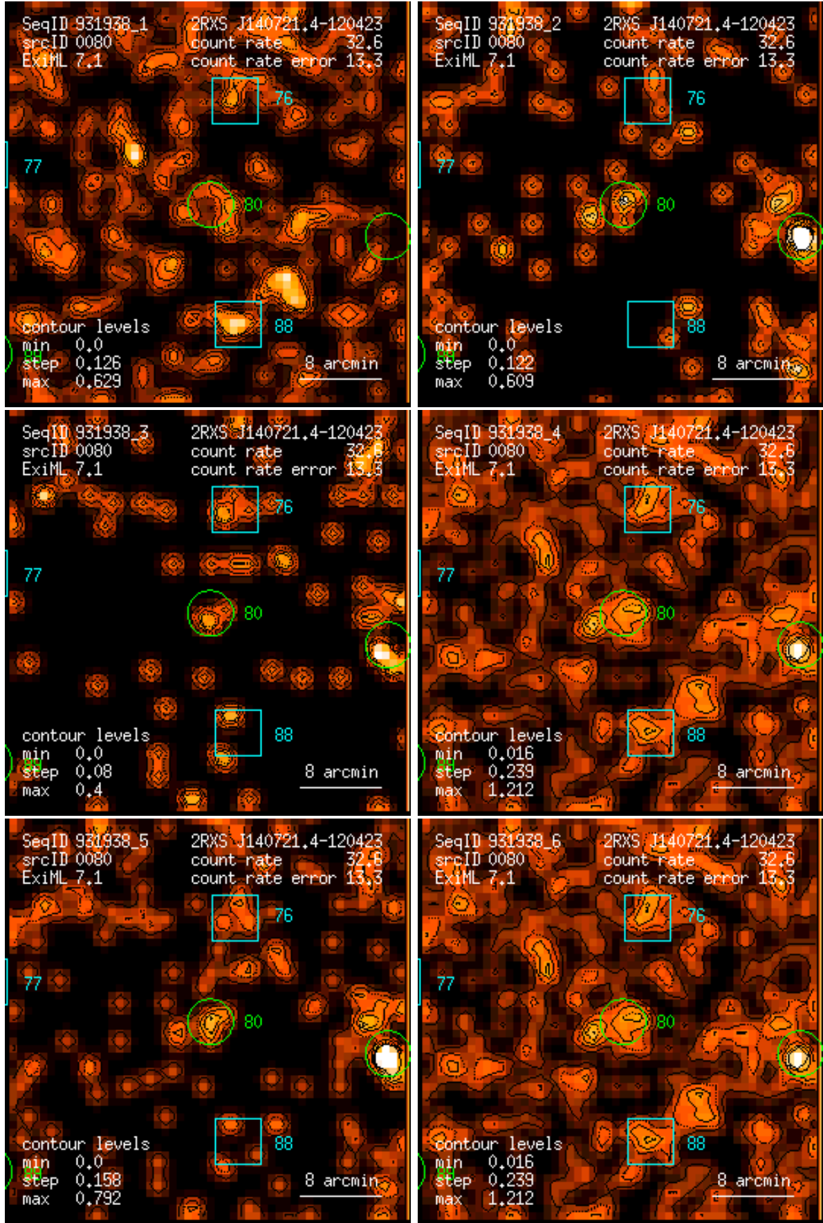
Figure 80: RASS 931938: detection 0080: band rate images, Gaussian filter: (1) PSPC channels 11 – 41, (2) 52 – 90, (3) 91 – 201, (4) 11 – 235, (5) 52 – 201, (6) 11 – 201. Broad band rates in counts/ks. Band rate contour levels in counts/ks/arcmin 2 .
