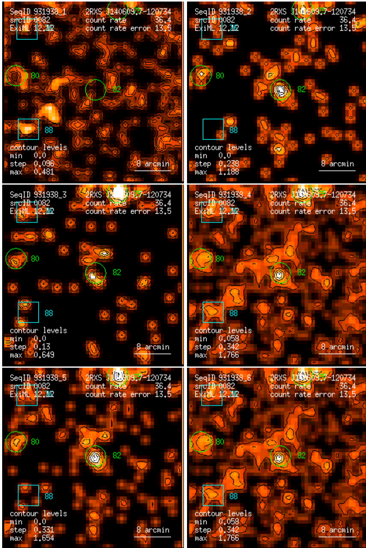
Figure 82: RASS 931938: detection 0082: band rate images, Gaussian filter: (1) PSPC channels 11 – 41, (2) 52 – 90, (3) 91 – 201, (4) 11 – 235, (5) 52 – 201, (6) 11 – 201. Broad band rates in counts/ks. Band rate contour levels in counts/ks/arcmin 2 .
