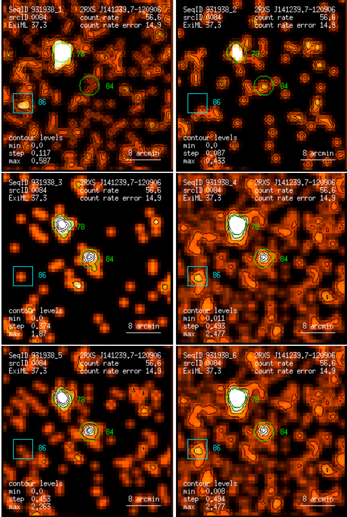
Figure 84: RASS 931938: detection 0084: band rate images, Gaussian filter: (1) PSPC channels 11 – 41, (2) 52 – 90, (3) 91 – 201, (4) 11 – 235, (5) 52 – 201, (6) 11 – 201. Broad band rates in counts/ks. Band rate contour levels in counts/ks/arcmin 2 .
