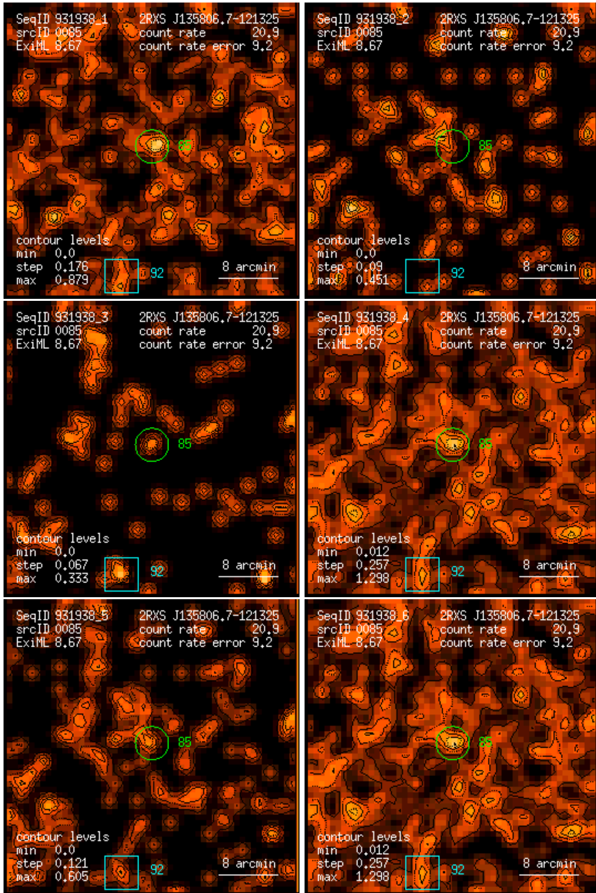
Figure 85: RASS 931938: detection 0085: band rate images, Gaussian filter: (1) PSPC channels 11 – 41, (2) 52 – 90, (3) 91 – 201, (4) 11 – 235, (5) 52 – 201, (6) 11 – 201. Broad band rates in counts/ks. Band rate contour levels in counts/ks/arcmin 2 .
