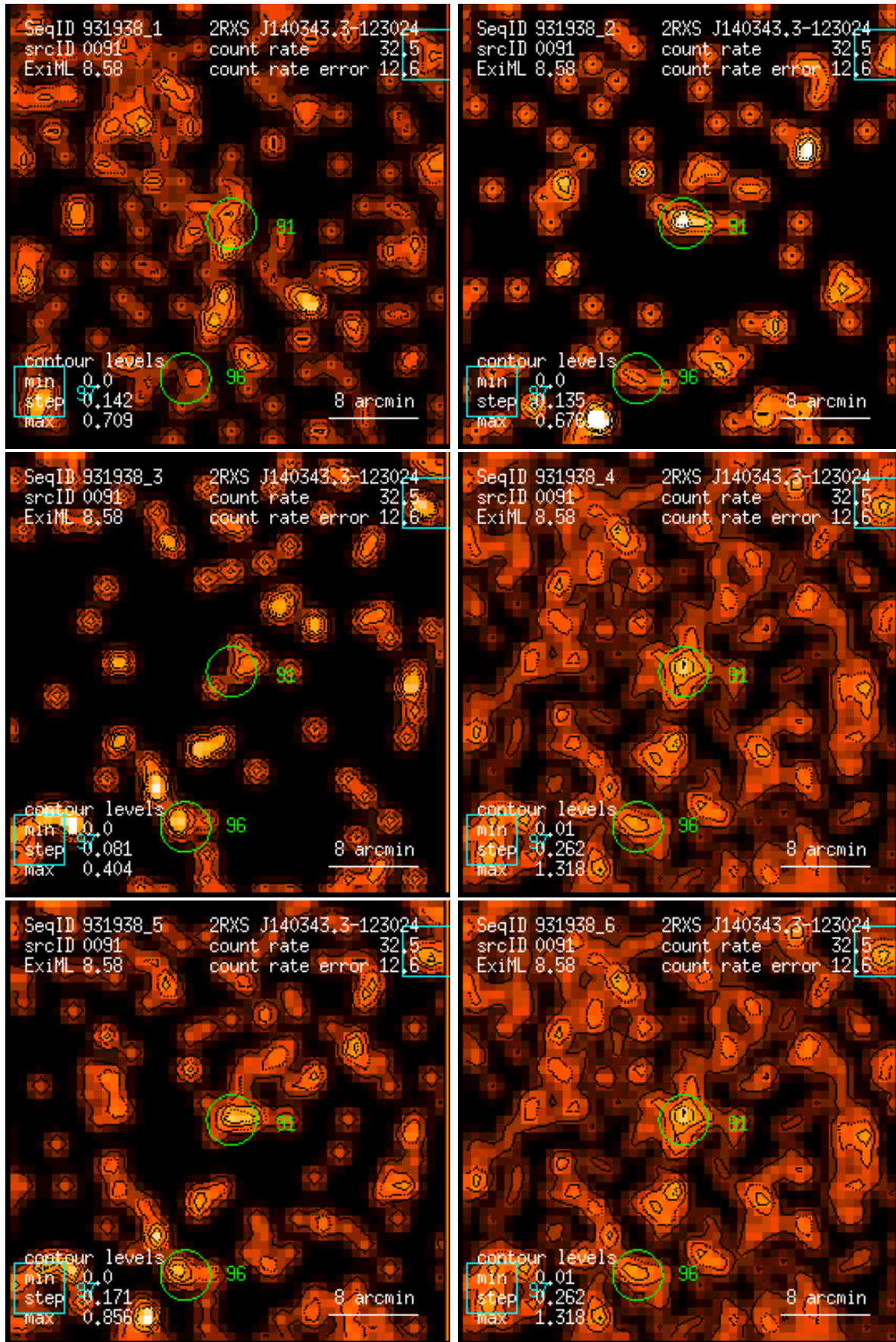
Figure 91: RASS 931938: detection 0091: band rate images, Gaussian filter: (1) PSPC channels 11 – 41, (2) 52 – 90, (3) 91 – 201, (4) 11 – 235, (5) 52 – 201, (6) 11 – 201. Broad band rates in counts/ks. Band rate contour levels in counts/ks/arcmin 2 .
