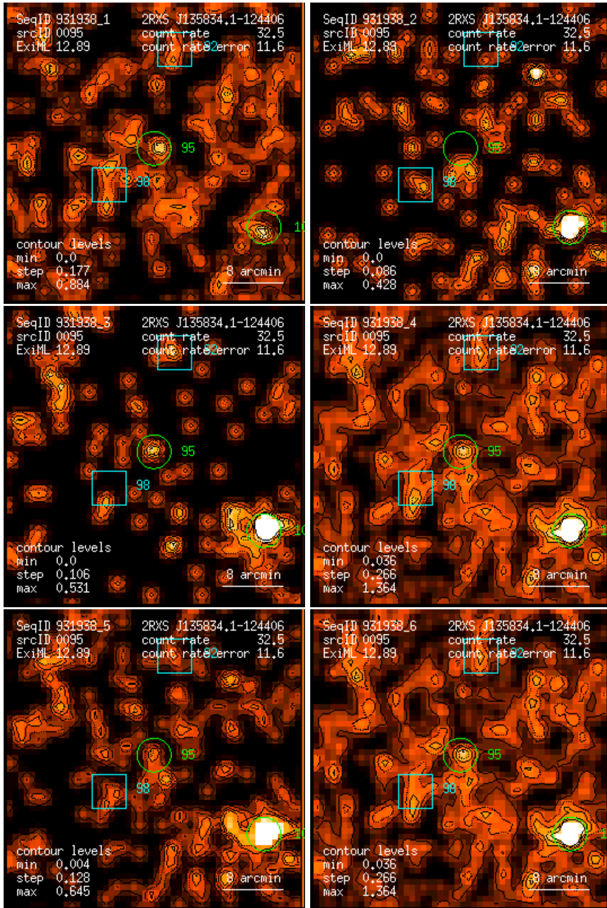
Figure 95: RASS 931938: detection 0095: band rate images, Gaussian filter: (1) PSPC channels 11 – 41, (2) 52 – 90, (3) 91 – 201, (4) 11 – 235, (5) 52 – 201, (6) 11 – 201. Broad band rates in counts/ks. Band rate contour levels in counts/ks/arcmin 2 .
