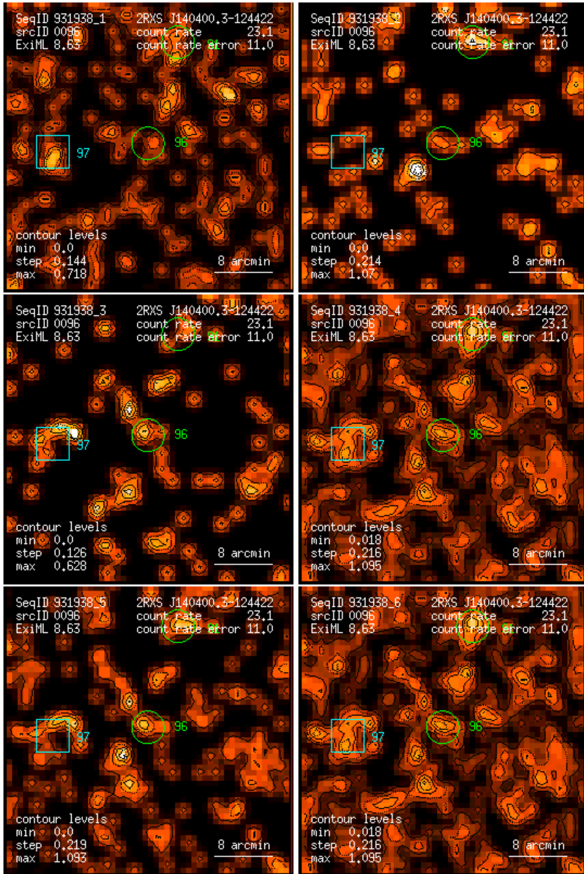
Figure 96: RASS 931938: detection 0096: band rate images, Gaussian filter: (1) PSPC channels 11 – 41, (2) 52 – 90, (3) 91 – 201, (4) 11 – 235, (5) 52 – 201, (6) 11 – 201. Broad band rates in counts/ks. Band rate contour levels in counts/ks/arcmin 2 .
