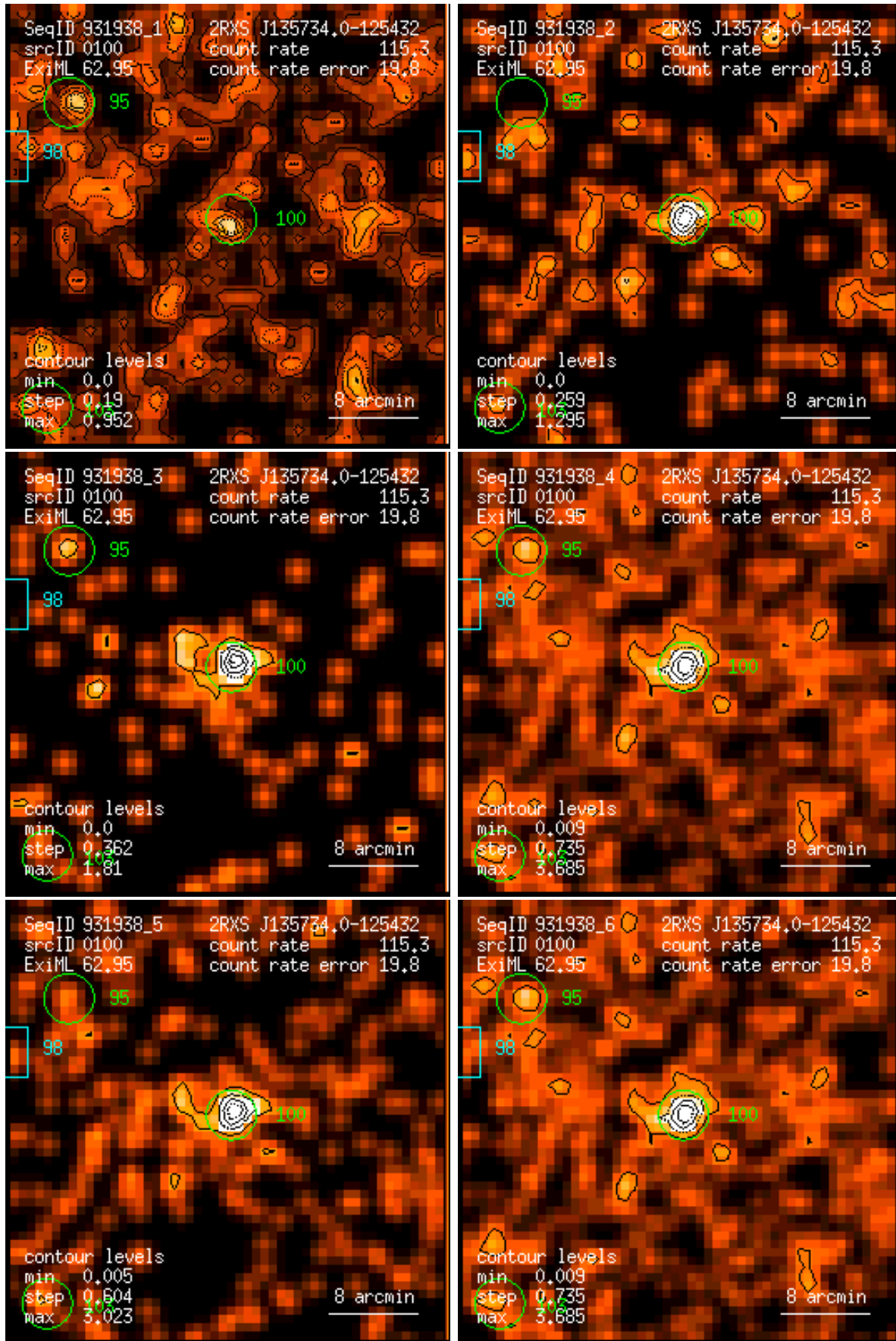
Figure 100: RASS 931938: detection 0100: band rate images, Gaussian filter: (1) PSPC channels 11 – 41, (2) 52 – 90, (3) 91 – 201, (4) 11 – 235, (5) 52 – 201, (6) 11 – 201. Broad band rates in counts/ks. Band rate contour levels in counts/ks/arcmin 2 .
