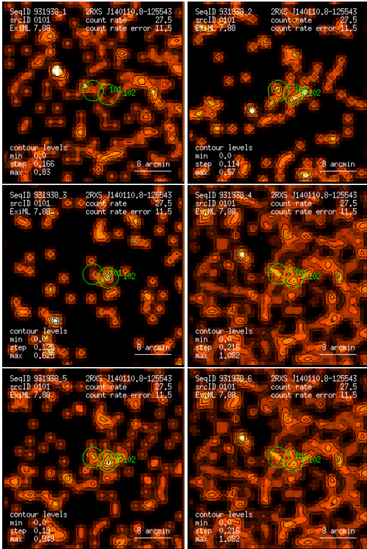
Figure 101: RASS 931938: detection 0101: band rate images, Gaussian filter: (1) PSPC channels 11 – 41, (2) 52 – 90, (3) 91 – 201, (4) 11 – 235, (5) 52 – 201, (6) 11 – 201. Broad band rates in counts/ks. Band rate contour levels in counts/ks/arcmin 2 .
