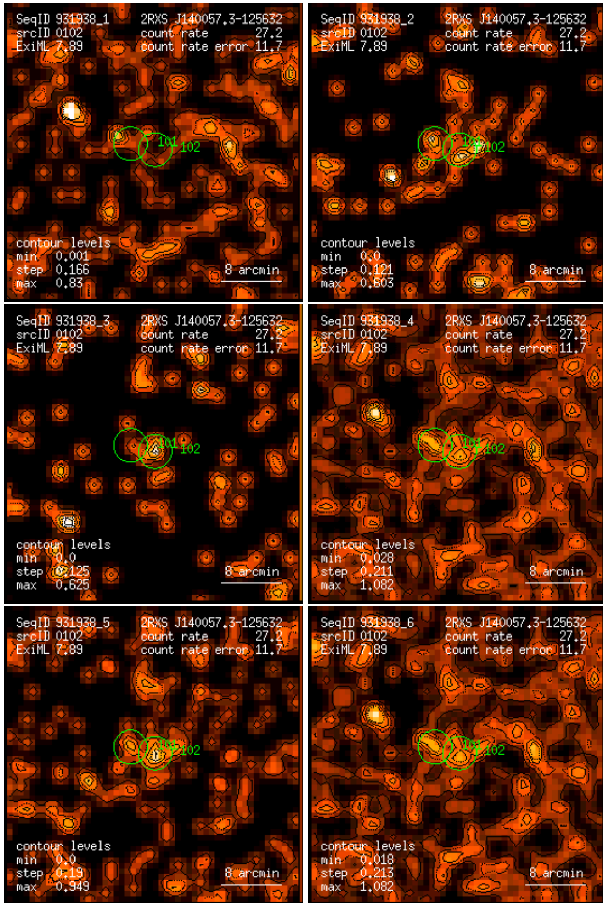
Figure 102: RASS 931938: detection 0102: band rate images, Gaussian filter: (1) PSPC channels 11 – 41, (2) 52 – 90, (3) 91 – 201, (4) 11 – 235, (5) 52 – 201, (6) 11 – 201. Broad band rates in counts/ks. Band rate contour levels in counts/ks/arcmin 2 .
